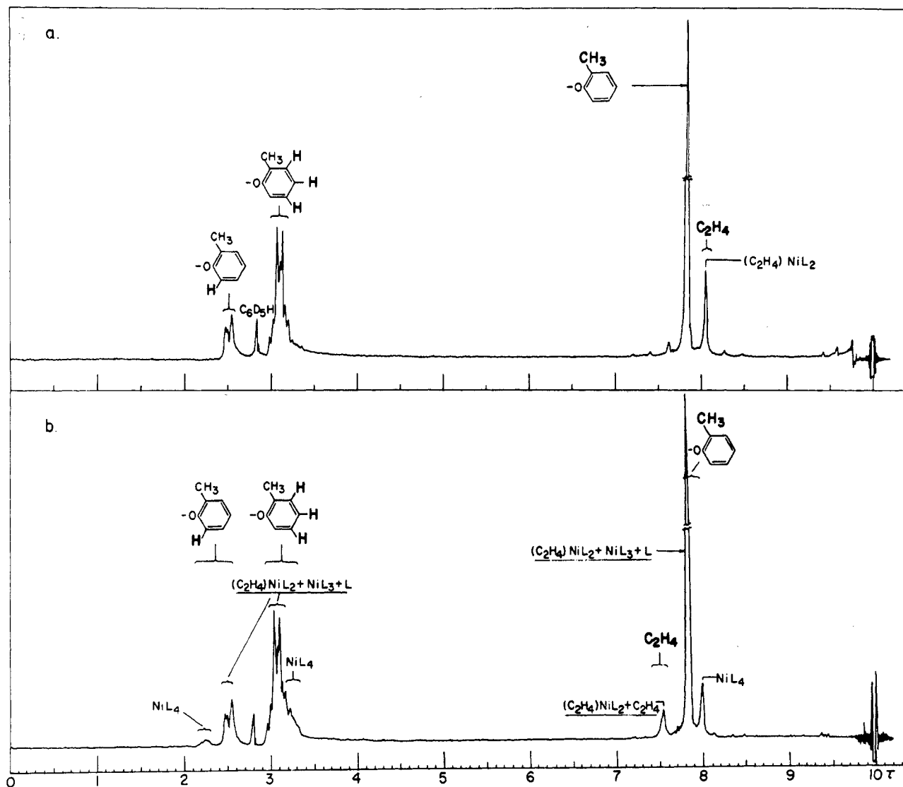
Figure 1.—The 100-Mc proton nmr spectrum of (a) 0.1 mmol of (\text{C}_2\text{H}_4)\text{Ni}[\text{P}(\text{O}-o\text{-C}_6\text{H}_4\text{CH}_3)_2]_2 in 0.4 ml of \text{C}_6\text{D}_6 solution and (b) the same solution with 0.1 mmol of \text{P}(\text{O}-o\text{-C}_6\text{H}_4\text{CH}_3)_3 added. Each resonance indicated by an underlined sum of species is an average caused by rapid exchange.
