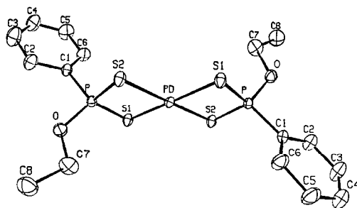
Fig. 1. A perspective view of the Pd(S 2 P(OEt)φ) 2 molecule with the labeling scheme. The atoms are represented by 30% probability thermal ellipsoids. The same labeling scheme was used for the platinum(II) compound.
