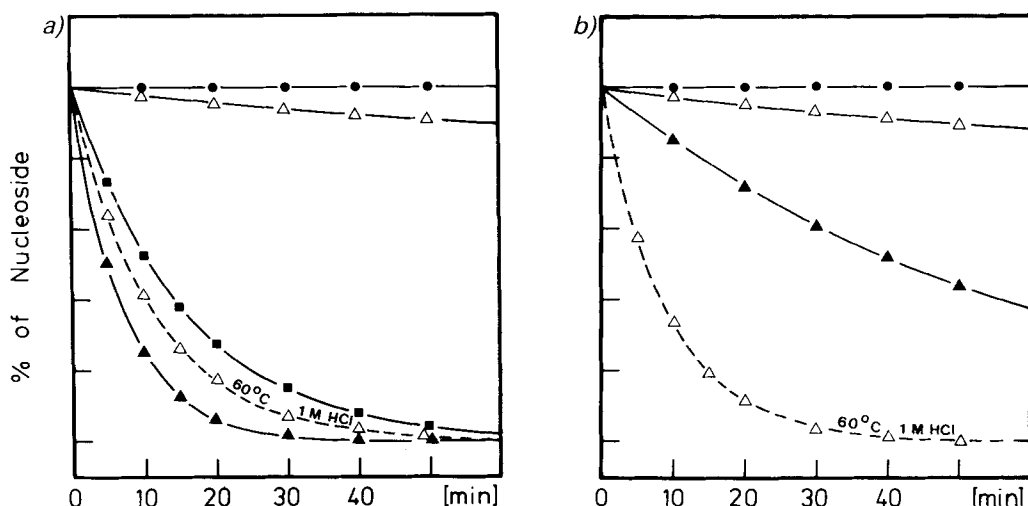
Fig. Hydrolyses rates of isosteric 2'-deoxyribofuranosides in 0.5 M HCl at 25°. Data are taken from the decrease of the UV absorption at the wavelength indicated: a) 3 at 260 nm (■—■), 4 at 270 nm (●—●), 1 at 251 nm (▲—▲), and 2 at 260 nm (△—△); b) 19 at 350 nm (●—●), 17a at 237 nm (▲—▲), and 18a at 345 nm (△—△).
