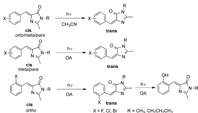
Scheme 2. Photoreactions of ortho , meta , and para Halogenated BMIs in Acetonitrile Solution and as Host–guest Complexes with OA in Water
