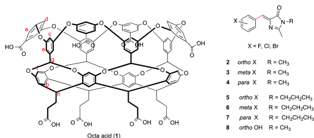
Scheme 1. Chemical Structure of Octa Acid (1) and Guest Molecules Studied
