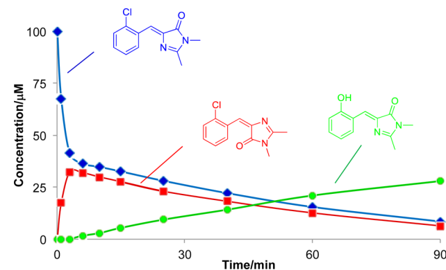
Figure 3. Phototransformation of cis-ortho -Cl/ N -Me@OA 2 (100 \mu\text{M} :200 \mu\text{M} ) in borate aqueous solution (10 mM) at pH 9, and formation of trans-ortho -Cl/ N -Me and cis-ortho -OH/ N -Me.
