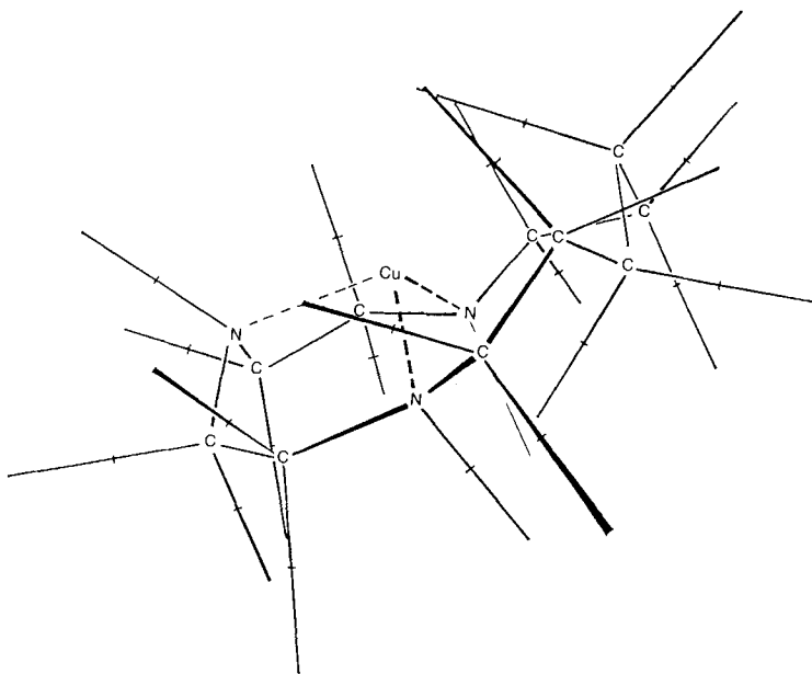
Fig. 2. Molecular model of [\text{CuL}]^+ from 5, indicating crowding at fourth coordination site
