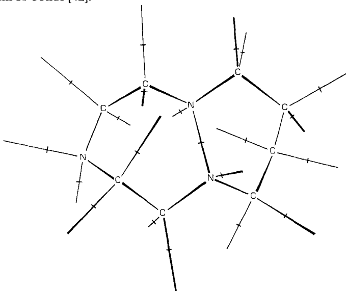
Fig. 1. Molecular model of H-bonded species \text{LH}_2 of 3 . Hydrogen van der Waals radii are indicated. \text{LH} is obtained by deprotonation of the non-bridgehead N-atom. The dash | indicates estimated position of H-atoms.
