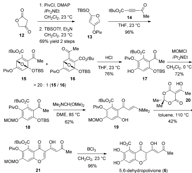
Scheme 4. Synthesis of 5,6-dehydropolivione ( 6 ) from tetronic acid ( 12 ). Piv = pivaloyl, DMAP = 4-(dimethylamino)pyridine, TBS = tert -butyldimethylsilyl, MOM = methoxymethyl, DME = 1,2-dimethoxyethane.
