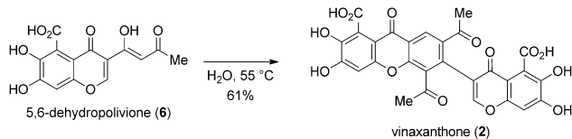
Scheme 5. Dimerization of 5,6-dehydropolivione ( 6 ) under neutral conditions to generate vinaxanthone ( 2 ).
