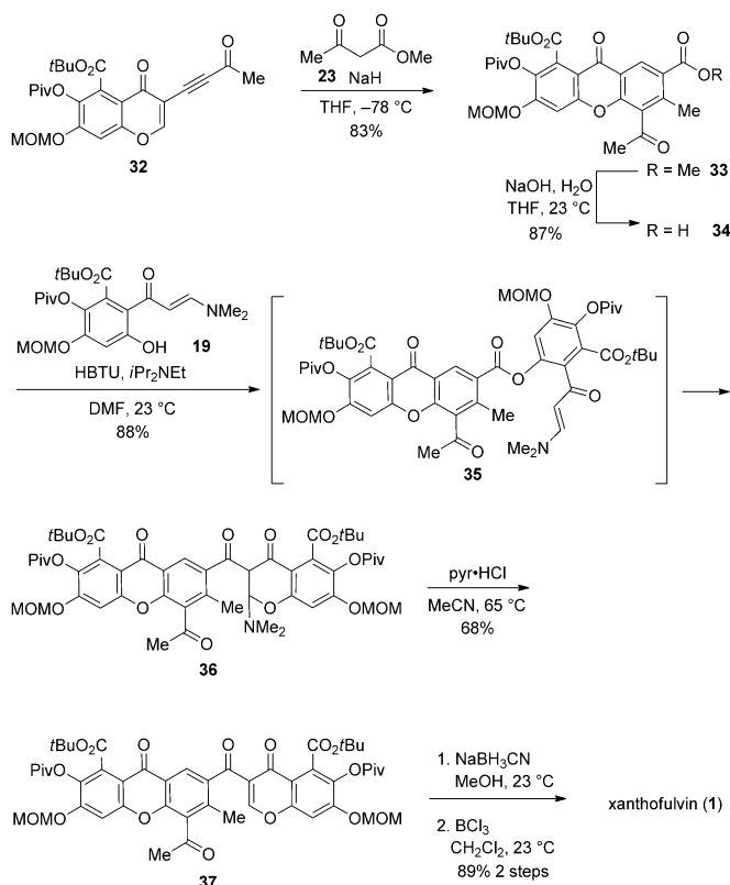
Scheme 8. Completion of the synthesis of xanthofulvin ( 1 ). HBTU = O -(1- H -benzotriazolyl-1-yl)- N,N,N,N '-tetramethyluronium hexafluorophosphate.
