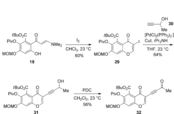
Scheme 7. Synthesis of ynone 32 . PDC = pyridinium dichromate.
