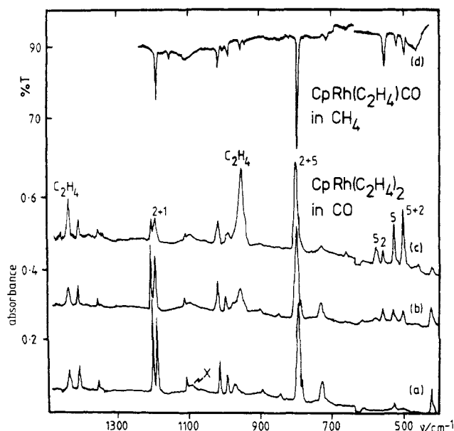
Figure 7. (a) IR spectrum of 1 in CO matrix (conditions as in Figure 5); (b) after 11 min of Hg arc photolysis; (c) after annealing to 38 K, recoling followed by a further 93 min of photolysis showing growth of bands of 2 , 5 , and \text{C}_2\text{H}_4 ; (d) spectrum of 2 deposited directly into a \text{CH}_4 matrix ( T_s = 249 K, t_d = 55 min, 4.2 mmol of \text{CH}_4 ).
