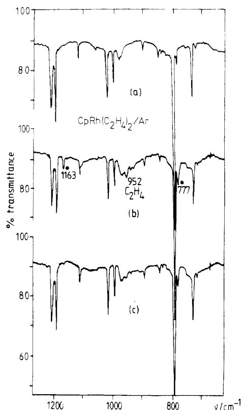
Figure 1. (a) Infrared spectrum of \text{CpRh}(\text{C}_2\text{H}_4)_2 ( 1a ) in argon at 20 K (sublimation temperature, T_s = 273 K, deposition time, t_d = 130 min, 4.2 mmol of Ar); (b) after 900 min of irradiation with Cd arc ( \lambda = 326 , 229 nm) showing growth of bands of \text{C}_2\text{H}_4 and 3 (●); (c) after a further 150 min of irradiation at \lambda = 436 nm showing partial reversal of reaction.
