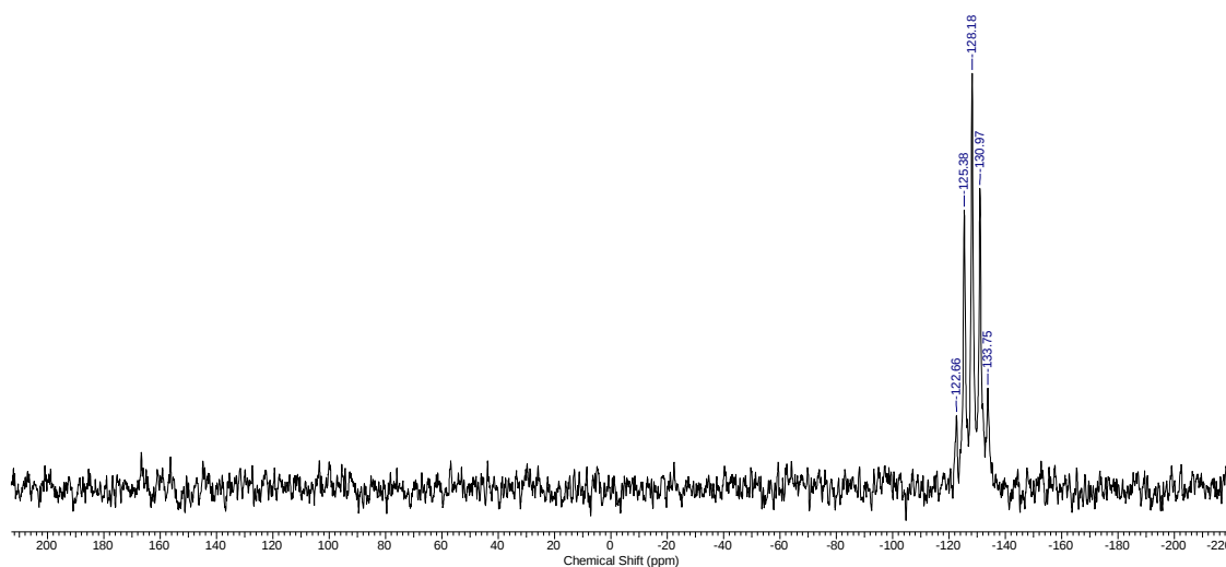
Figure S2. ^{119}\text{Sn} NMR spectrum ( \text{CDCl}_3 , 298 K) of 8 .
