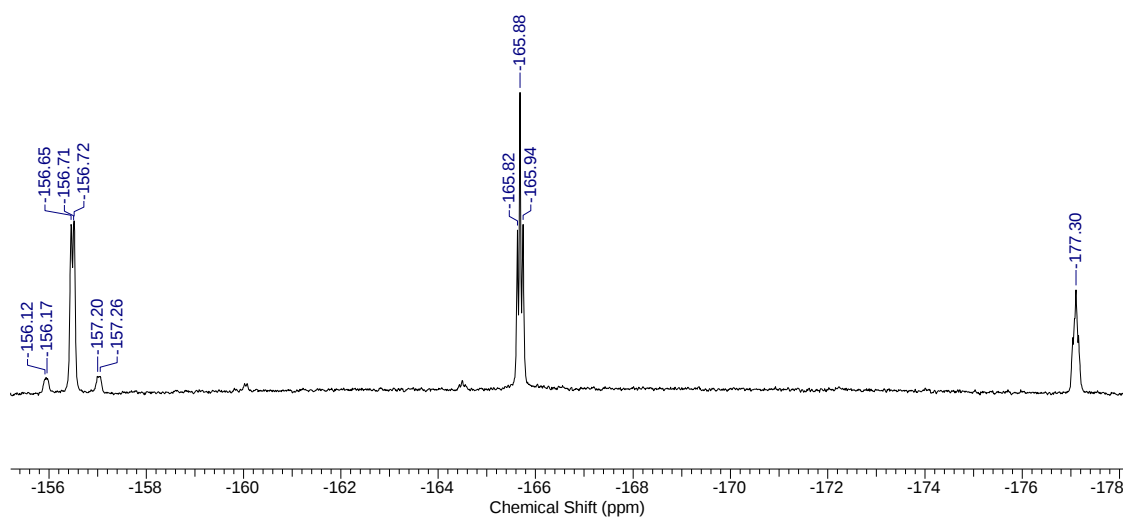
Figure S1. ^{19}\text{F} NMR spectrum ( \text{CDCl}_3 , 298 K) of complex 8 .
