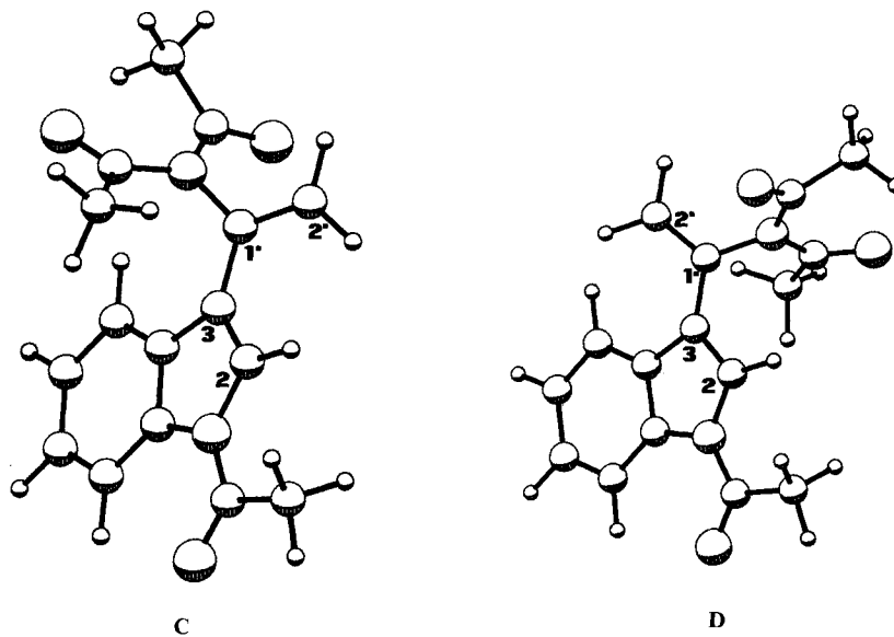
Fig.1. Energy minimum conformations of 1c calculated by molecular mechanics 23 . C = s-cis-synclinal conformer, torsional angle C(2)-C(3)-C(1')-C(2') = 30^\circ ; D = s-trans-synclinal conformer, torsional angle C(2)-C(3)-C(1')-C(2') = -144^\circ . The starting geometry was taken from an X-ray analysis of conformer I (Table).
