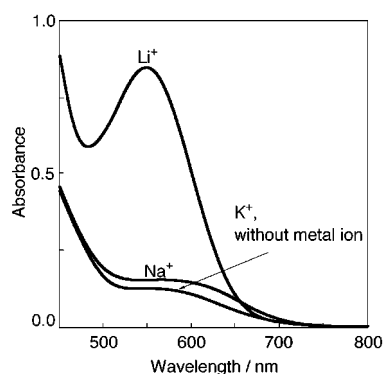
Fig. 1 Absorption spectra of crowned spirobenzothiopyran 1 under UV irradiation in the absence and presence of an alkali metal ion. 1 and alkali metal perchlorate: 2 \times 10^{-4} \text{ mol dm}^{-3} in acetonitrile.
