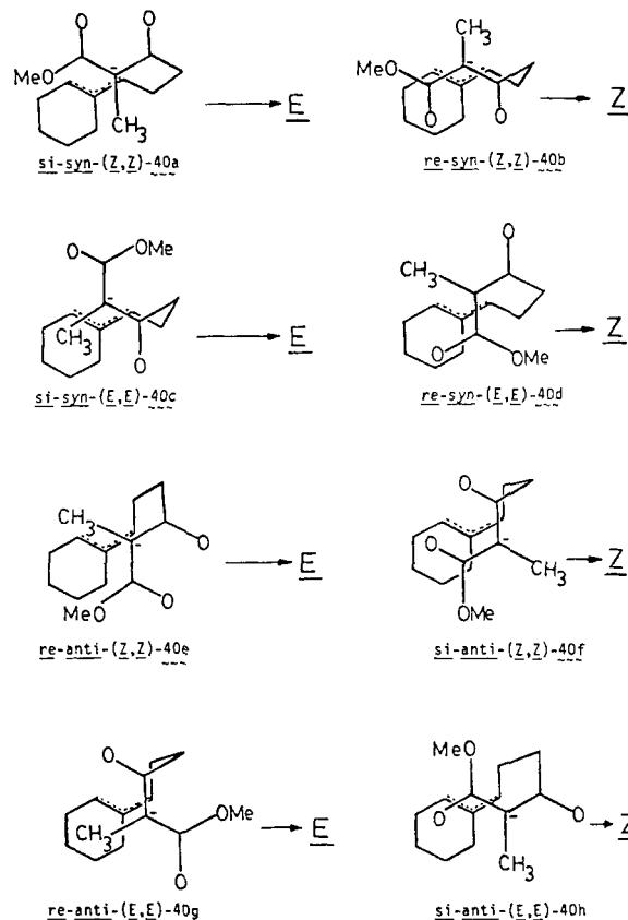
Scheme IV. Transition States for Formation of 31 and 32
