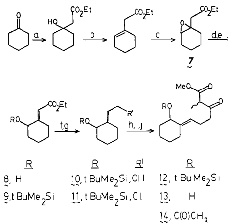
Scheme I. Synthesis of (E)-2-Acetoxy[[3-oxo-4-(carbomethoxy)-pentyl]methylidene]cyclohexane
