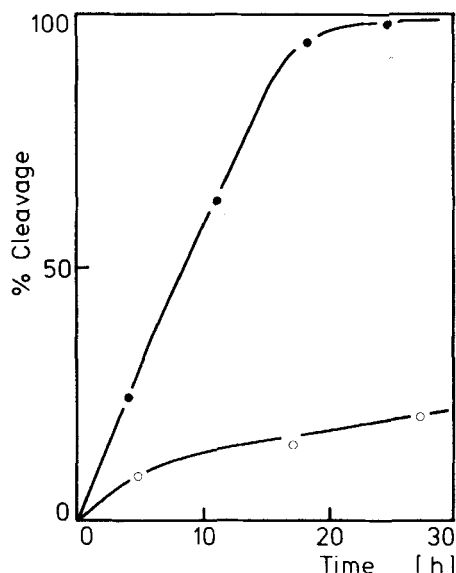
Fig. 4. Time course of phosphodiester hydrolysis of the oligomers d (A-T-G-A-A-G-C-T-T-C-A-T) ( 10 ); ● and d (A-T-G-A- m 6 A-G-C-T-T-C-A-T) ( 14 ); ○ on treatment with the endodeoxyribonuclease Hind III. For conditions, see Exper. Part .
