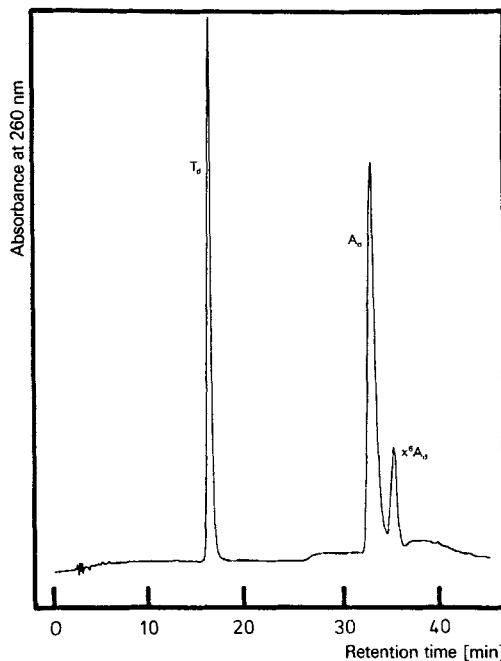
Fig. 2. HPLC profile of phosphodiester-hydrolysis products of the oligomer 8 after treatment with snake-venom phosphodiesterase and alkaline phosphatase. Conditions, see Exper. Part ; x^*A_0 = N^6 -(carbamoylmethyl)-2'-deoxyadenosine ( 1 ).
