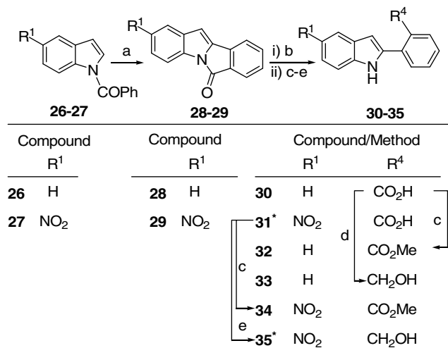
Scheme 4. Reagents and conditions: (a) Pd(OAc) 2 , AcOH, 110 °C; 20 (b) tBuOK, tBuOH/H 2 O, 82 °C; 20 (c) AcCl, MeOH, reflux; (d) LiAlH 4 , THF, rt; (e) BH 3 -THF, rt. 13 *Compounds synthesized previously. 13
