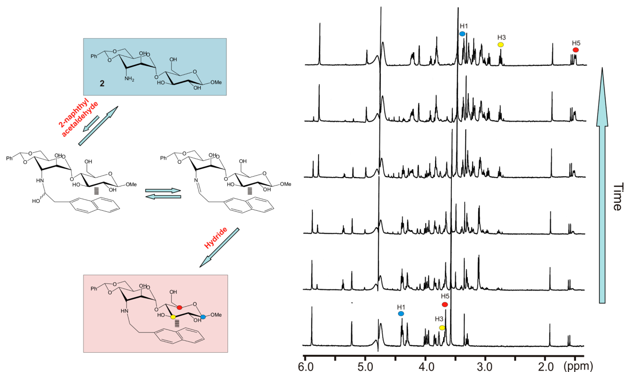
Figure 3. Reductive amination reaction performed with disaccharide 2 and 2-naphthylacetaldehyde in D 2 O (10 mM phosphate, pH 6.2). The time evolution of the reaction mixture is represented at the right. Key signals of the glucose unit that were shifted upfield (by up to 2.12 ppm) because of the proximity of the naphthyl ring are highlighted.
