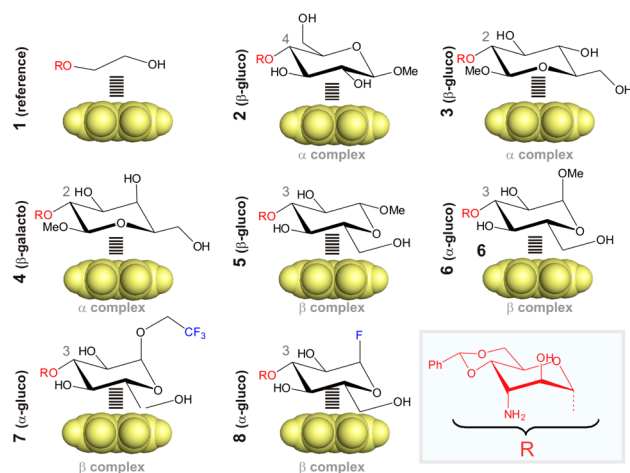
Figure 2. Representation of the synthesized disaccharide library. The configuration of the interacting pyranoses is indicated. Carbon positions involved in the glycosidic bonds are labeled in gray. Finally, carbohydrate/aromatic contacts formed upon reaction with 2-naphthylacetaldehyde are also shown.
