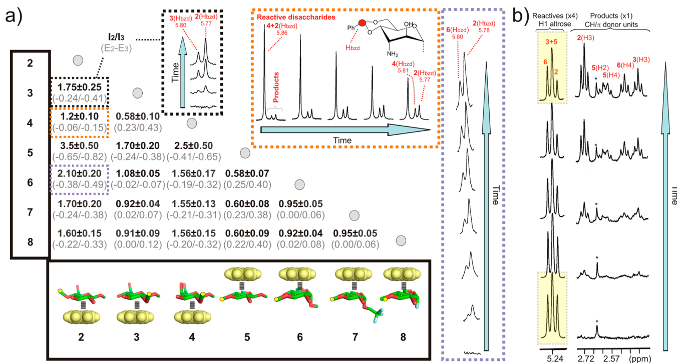
Figure 4. (a) Pairwise competition experiments performed with the library described herein. Equimolecular mixtures of two disaccharides in D 2 O (10 mM phosphate, pH 6.2) were treated with substoichiometric amounts of 2-naphthylacetaldehyde. After a short equilibration period, the reductive amination reactions were carried out by adding sodium cyanoborohydride. The ratio of secondary amine products obtained for each disaccharide pair ( I_x/I_y ) is indicated. These values were taken as indicators of the free energy differences between the alternative stacking modes ( E_x - E_y , in kcal/mol). Dotted boxes highlight the formation of the reaction products for pairs 2/3 , 2/4 , and 2/6 as revealed by NMR spectroscopy. For each signal, the compound number (in bold), proton assignment (in brackets), and chemical shifts in ppm are indicated. (b) Competition experiment performed with a 1:1:1:1 mixture of 2 , 3 , 5 , and 6 . Representative NMR signals for the disaccharide models and reaction products are shown. The compound numbers (in bold) and proton assignments (in brackets) are indicated.
