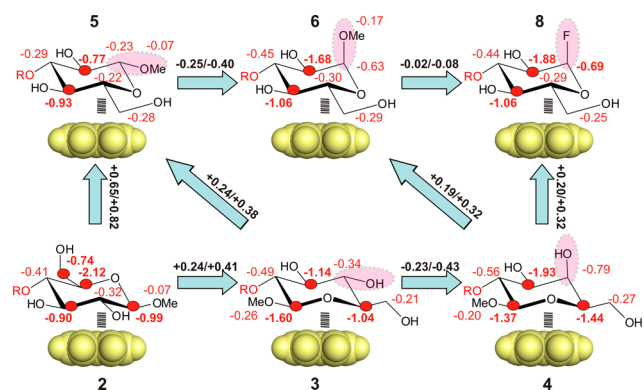
Figure 5. Stability differences for stacking complexes. Chemical shift perturbations promoted by the aromatic ring at the interacting D-pyranose unit in the reaction products are shown. For derivatives 3–8, the key positions 1 and 4 in the \beta and \alpha complexes, respectively, are highlighted in purple.
