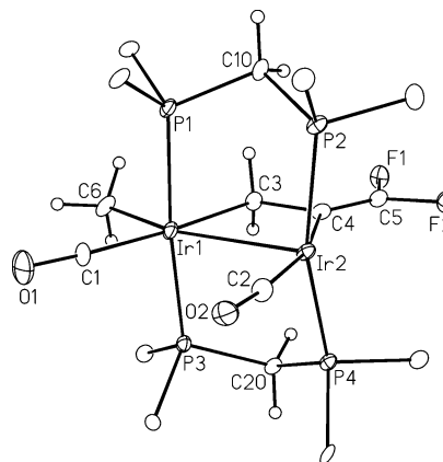
Figure 2. Perspective view of the [\text{Ir}_2(\text{CH}_3)(\text{CO})_2(\mu\text{-}\eta^1\text{:}\eta^1\text{-CH}_2=\text{C}=\text{CF}_2)(\text{dppm})_2]^+ cation of compound 5c . Thermal ellipsoids as for Figure 1. Only the ipso phenyl carbons are shown.
