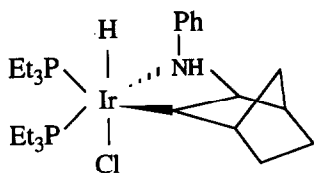
Fig. 2. Aziridacyclobutane complex occurring in iridium-catalysed condensation of aniline on norbornene.
