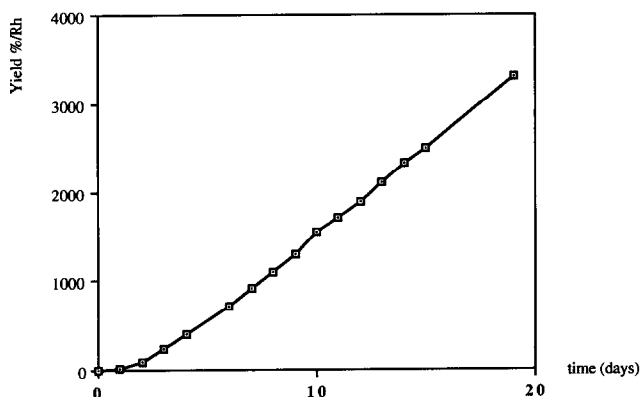
Fig. 1. Reaction yield for the condensation of aniline with norbornene in aniline as solvent.
