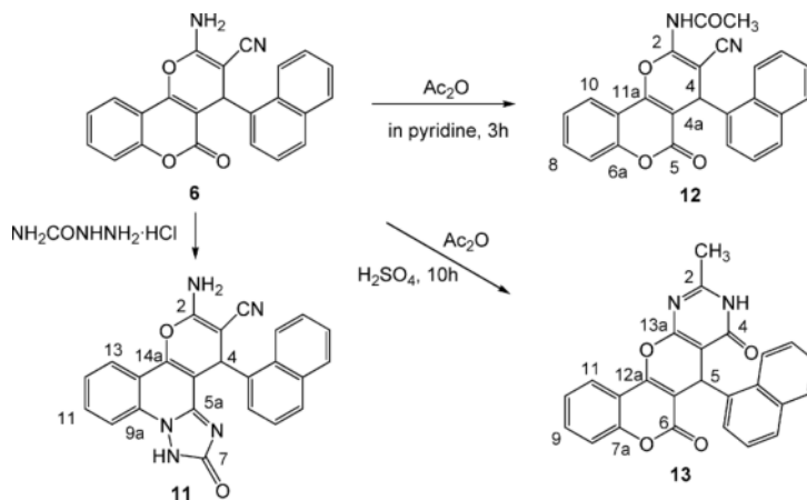
Scheme 2. Synthesis of [1,2,4]triazolo[1,5- a ]quinoline-11-carbonitrile ( 11 ), chromen-2-yl-acetamide ( 12 ), and chromeno-[3',4':5,6]pyrano[2,3- d ]pyrimidine-dione ( 13 ) derivatives.
