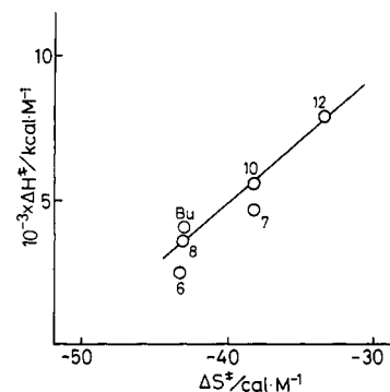
Figure 13. \Delta H^* - \Delta S^* compensation relationship.
