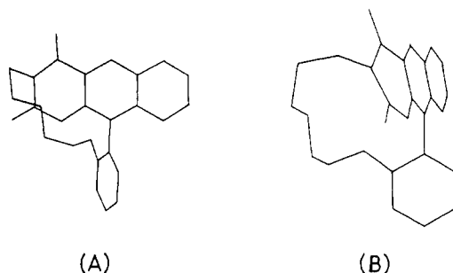
Figure 5. X-ray structure of dFl(6). In (A) the least-squares plane of the isoalloxazine ring is placed in the sheet plane. In (B) the 10-phenyl ring is placed in the sheet plane.
