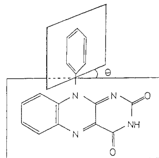
Figure 6 indicates the ab initio MO calculation of 10-phenylisoalloxazine plotted against \theta . It is seen from Figure 6
