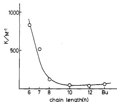
Figure 12. Equilibrium constants ( K ) for the reaction of FI( n ) and \text{Na}_2\text{SO}_3 .
