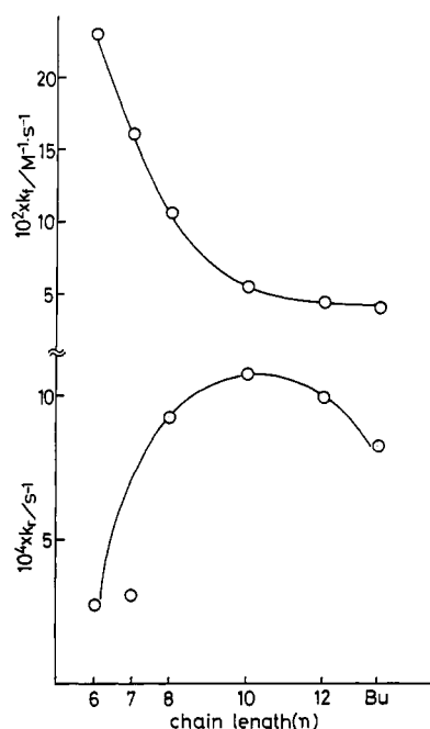
Figure 11. Forward rate constants ( k_f ) and reverse rate constants ( k_r ) for the reaction of FI( n ) and \text{Na}_2\text{SO}_3 .
