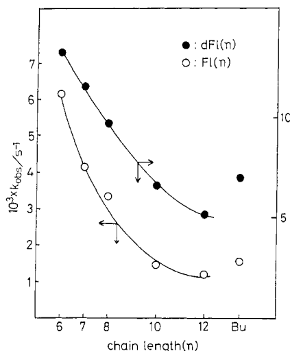
Figure 10. Pseudo-first-order rate constants ( k_{\text{obs}} ) for the reactions of FI( n ) and \text{Na}_2\text{SO}_3 (open circles) and of dFI( n ) and KCN (filled circles): 30 °C, aerobic, water/MeOH (50.8:49.2 v/v), [FI( n )] = (2.1\text{--}2.6) \times 10^{-5} M, [dFI( n )] = (2.2\text{--}2.6) \times 10^{-5} M, [ \text{Na}_2\text{SO}_3 ] = 3.00 \times 10^{-2} M, and [KCN] = 2.00 \times 10^{-3} M.
