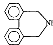
3,4,5,6-Dibenzohomopiperidine (XVIII)
