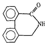
3,4,5,6-Dibenzohomopiperidin-2-one (XVII)
