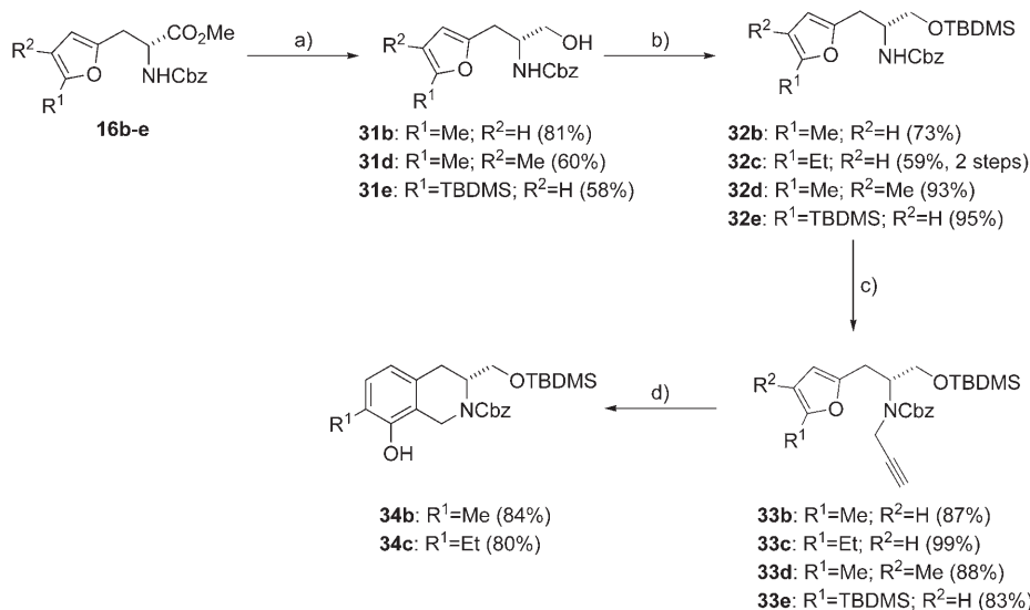
Scheme 8. Synthesis of the Cbz-protected substrates 33b–e and 34b–c . Reaction conditions: a) DIBAL-H, THF, -78^{\circ}\text{C} \rightarrow \text{RT} ; b) TBDMSCl, imidazole, DMF, RT; c) \text{BrCH}_2\text{C}\equiv\text{CH} , NaH, DMF, RT; d) [\mu\text{-Cl}(\text{AuPPh}_3)_2]\text{BF}_4 , \text{CDCl}_3 , RT.
