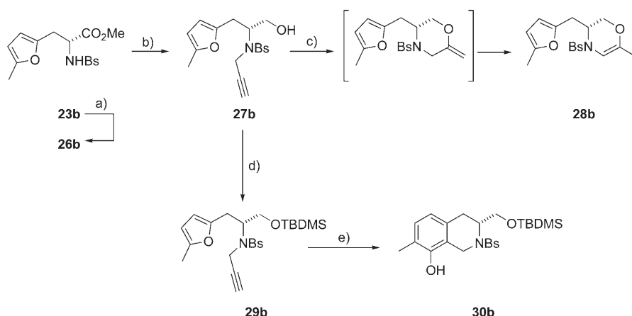
Scheme 7. The unprotected alcohol leads to 28b , while the protected one delivers 30b . Reaction conditions: a) DIBAL-H, THF, -78^\circ\text{C} \rightarrow \text{RT} ; b) \text{BrCH}_2\text{C}\equiv\text{CH} , \text{Cs}_2\text{CO}_3 , acetone, RT, \Sigma 77\% ; c) \text{AuCl}_3 (5 mol%), \text{CD}_3\text{CN} , RT, 99%; d) TBDMSCl, imidazole, DMF, RT, 66%; e) [\mu\text{-Cl}(\text{AuPPh}_3)_2]\text{BF}_4 , \text{CDCl}_3 , RT, 70%.
