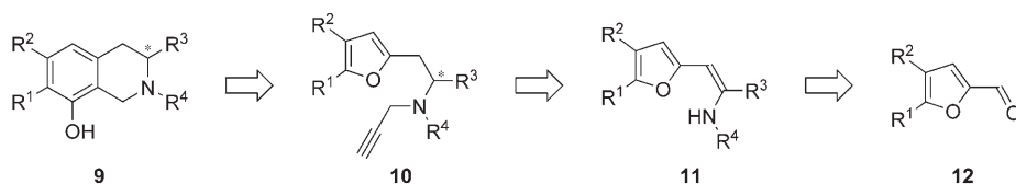
Scheme 3. Retrosynthesis of chiral 8-hydroxytetrahydroisoquinolines 9 .
