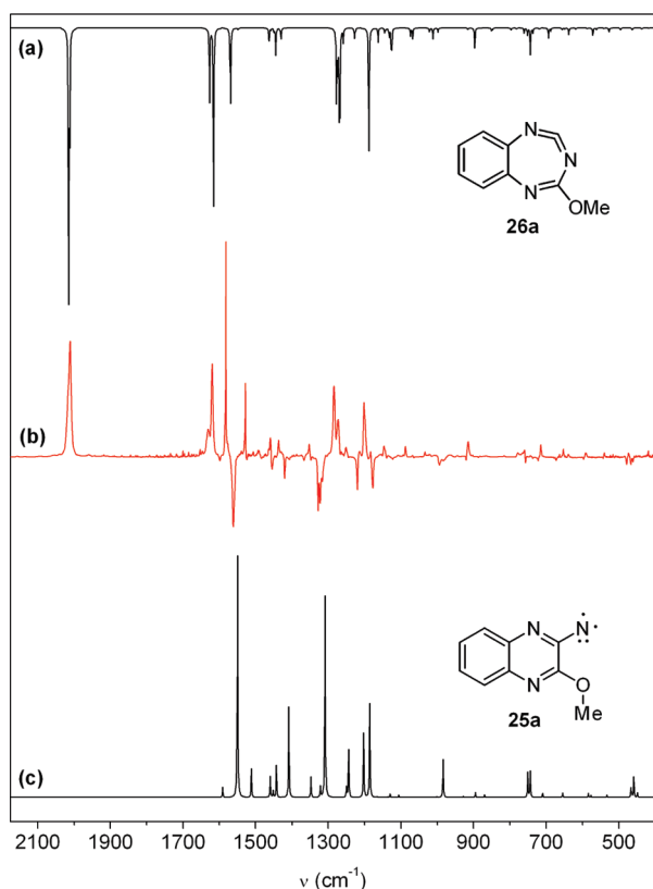
Figure 6. (a) IR spectrum of cyclic carbodiimide 26a calculated for a 3:1 mixture of the s -Z and s -E conformers; the calculated energy differences between these two conformers is 3.5 kcal/mol in favor of the s -Z conformer. (b) Ar matrix photolysis of 2-azido-3-methoxyquinoxaline 24Aa at 308 nm for 9 min (generating 3-methoxy-2-quinoxalinylnitrene 25a (not shown; cf. UV spectrum in Figure S13) followed by photolysis at \lambda > 434 nm (cutoff filter) for 2 min. Positive bands, carbodiimide 26a ; negative bands, nitrene 25a . (c) Calculated IR spectrum of nitrene 25a (B3LYP/6-31G**); wavenumbers scaled by a factor 0.9613). Ordinates in arbitrary absorbance units.
