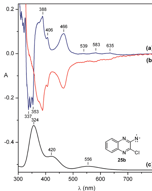
Figure 7. (a) UV-vis difference spectrum from the photolysis of the 2-azido-3-chloroquinoxaline 24Ab (negative bands 337–353 nm) at 308 nm for 90 s, showing appearance of the nitrene (positive bands). (b) Difference spectrum from photobleaching the nitrene at 395–460 nm for 16 min (photolysis >640 nm results in an analogous but weaker spectrum). (c) Calculated spectrum by TD-B3LYP/6-31+G** convoluted using the SWizard program. 11
