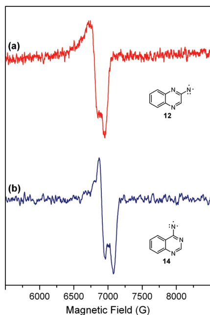
Figure 1. Quinoxalinylnitrenes and Quinazolinynitrenes. (a) Photolysis of tetrazoloquinoxaline 11T /2-azidoquinoxaline 11A at 308 nm for 2 min. 2-Quinoxalinylnitrene 12 : X_2 = 6820 G, Y_2 = 6965 G, H_0 = 3468.3 G, \nu = 9.720 GHz G; D/hc = 0.9538 \pm 0.0025 , E/hc = 0.0030 \pm 0.0001 cm ^{-1} (average of three experiments). (b) Photolysis of tetrazoloquinazoline 13T /4-azidoquinazoline 13A at 308 nm for 5 min. 2-Quinazolinynitrene 14 : H_0 = 3468.3 G, 6911 G, Y_2 = 7077 G, H_0 = G , \nu = 9.720 GHz, X_2 = 6911 , Y_2 = 7077 G, \Delta m_s = 2 : 1550 G; D/hc = 0.9934 \pm 0.0016 , E/hc = 0.0034 \pm 0.0001 cm ^{-1} (average of three experiments).
