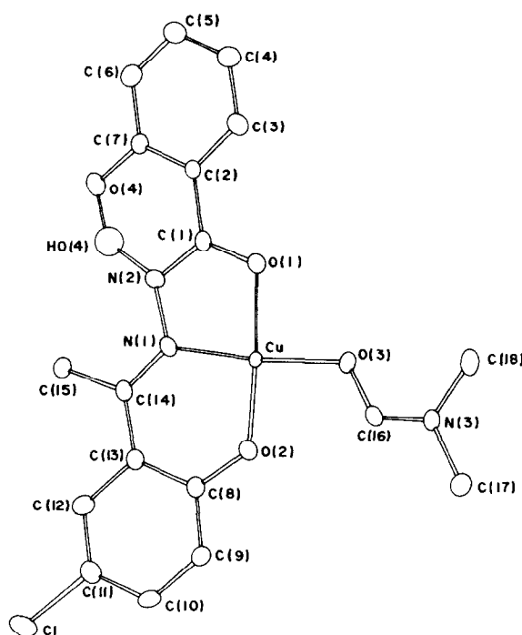
Fig. 1. ORTEP drawing showing the atom-numbering scheme for Cu(5Cl-OHA-SHZ) DMF.
