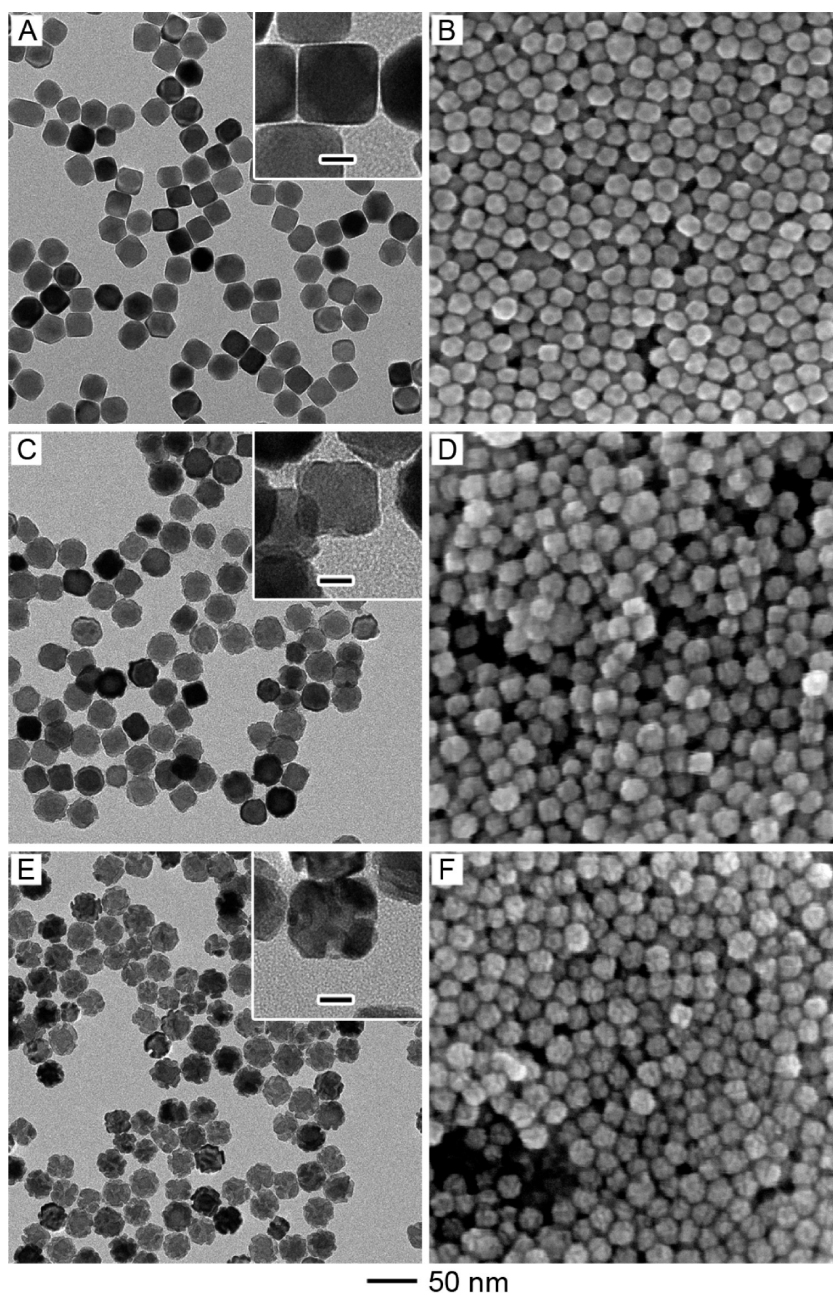
Figure 6. (A) TEM and (B) SEM images of Pd cuboctahedrons with an average edge length of 25 nm. (C and E) TEM and (D and F) SEM images of concave Pd–Pt cuboctahedrons synthesized at 90 °C for 12 h, with 1.4 and 3.5 mg of \text{H}_2\text{PtCl}_6 being added, respectively. The insets show TEM image of individual nanocrystals at a higher magnification. The scale bars in the insets are 10 nm.
