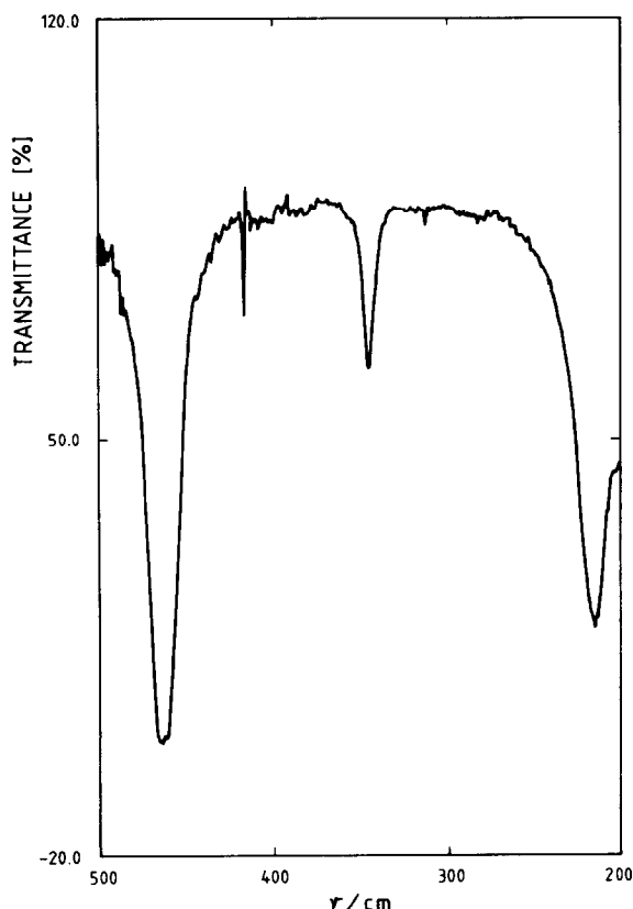
Fig. 9. Far infra-red spectra of toluene measured in a 0.1 mm CsJ cell.
