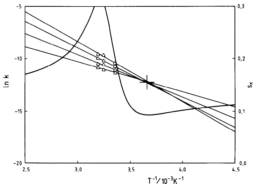
Fig. 6. Arrhenius plot for the thermal isomerization of triphenylformazanes in toluene, process B; compounds 2, 3, 6 and 8. Curved line refers to sum of squares of deviations of constrained straight lines from measurement points.
