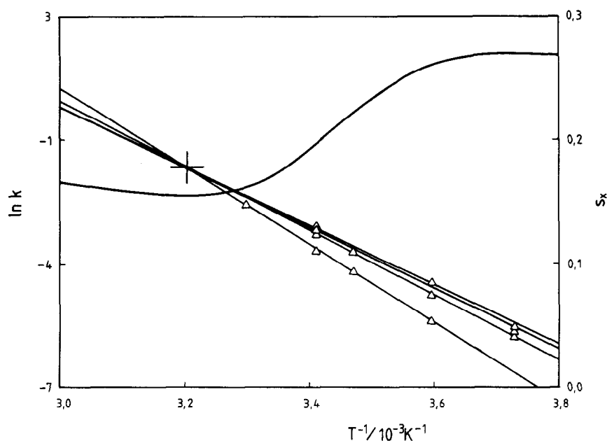
Fig. 5. Arrhenius plot for the thermal isomerization of triphenylformazanes in toluene: process A; compounds 6, 8, 9 and 10. The curved line refers to the sum of squares of deviations of constrained straight lines from measurement points.
