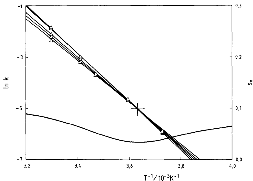
Fig. 4. Arrhenius plot for the thermal isomerization of triphenylformazanes in toluene: process A; compounds 1 to 5. The curved line refers to the sum of squares of deviations of constrained straight lines from measurement points.
