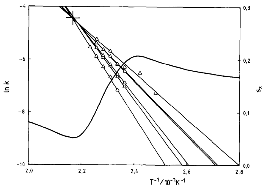
Fig. 2. Arrhenius plot for the thermal decomposition of nitroethyl-benzoates. The curved line refers to the sum of squares of deviations of constrained straight lines from measurement points.
