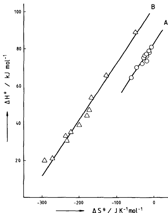
Fig. 3. \Delta H^\ddagger:\Delta S^\ddagger plot for the thermal isomerization of triphenylformazanes in toluene: process A ( \circ ) and process B ( \triangle ).
