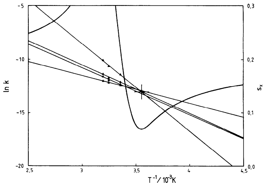
Fig. 8. Arrhenius plot for the thermal isomerization of triphenylformazanes in toluene, process B; compounds 1, 5, 7 and 11. Curved line refers to sum of squares of deviations of constrained straight lines from measurement points.
