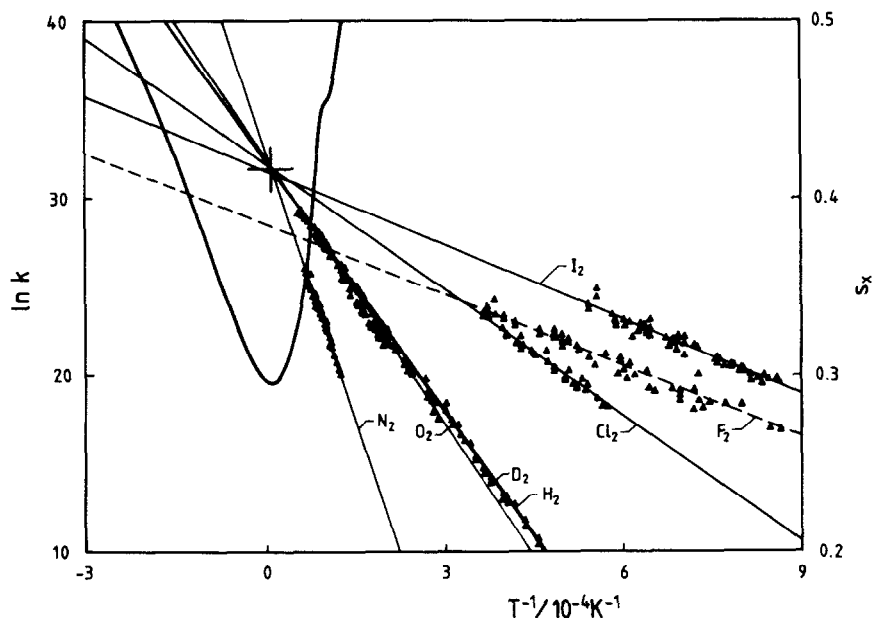
Fig. 1. Arrhenius plots for thermal dissociation of homonuclear diatomic gases highly diluted in argon. The curved line refers to the sum of squares of deviations of constrained straight lines from measurement points.
