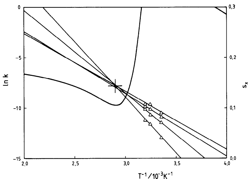
Fig. 7. Arrhenius plot for the thermal isomerization of triphenylformazanes in toluene, process B; compounds 7, 8, 9 and 10. Curved line refers to sum of squares of deviations of constrained straight lines from measurement points.
