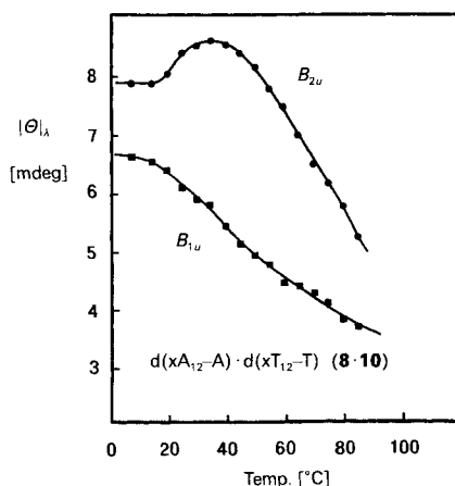
Fig. 3. Temperature-dependent ellipticities |\theta| of the B_{1u} and B_{2u} transition of d[(xA)_{12}\text{-}A] \cdot d[(xT)_{12}\text{-}T] ( 8 · 10 ; oligomer conc., 2.2 \mu\text{M} of single strands, buffer, see Fig. 1)
