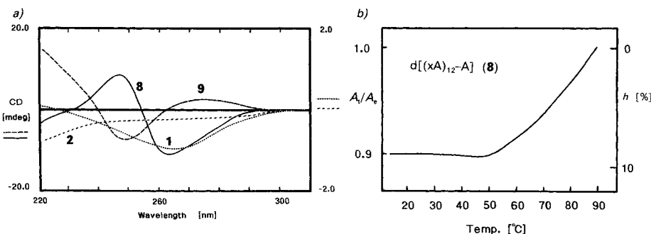
Fig. 1. a) CD Spectra of d[(xA)_{12}\text{-}A] ( 8 ) and d(A_{12}) ( 9 ; left-hand scale) and of A_d ( 1 ) and xA_d ( 2 ; right-hand scale; oligomer conc., 1.1 \mu M ; monomer conc., 25.9 \mu M ; measured in 60 mM cacodylate buffer (pH 7.0, 1M NaCl, 100 mM MgCl_2 ), at 8°) and b) normalized melting profile of d[(xA)_{12}\text{-}A] ( 8 ; conc., 1.3 \mu M ; buffer, see Fig. 1)
