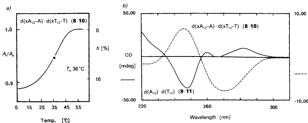
Fig. 2. a) Normalized melting profile of d[(xA)_{12}-A] \cdot d[(xT)_{12}-T] ( 8·10 ; oligomer conc., 0.8 \mu M of double strand; buffer, see Fig. 1) and b) CD spectra of d(A_{12}) \cdot d(T_{12}) ( 9·11 ; left-hand scale) and d[(xA)_{12}-A] \cdot d[(xT)_{12}-T] ( 8·10 , right-hand scale; oligomer conc., 2 \mu M of single strands, each; at 15°; buffer, see Fig. 1)
