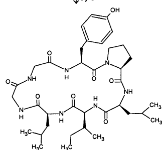
Pseudostellarin D (7)
