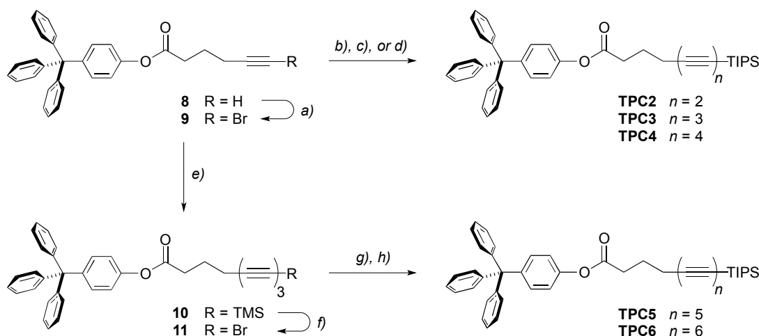
Scheme 2. Synthesis of oligoynes tritylphenyl carboxylates TPC2-6 up to the hexaynes. Reagents and conditions: a) \text{AgNO}_3 , NBS, DCM/MeCN, 96%; b) \text{TIPS-C}\equiv\text{C-ZnCl } \mathbf{1} , \text{PdCl}_2(\text{dppf}) \cdot \text{DCM} , THF/toluene, 68%; c) \text{TIPS-(C}\equiv\text{C)}_2\text{-ZnCl } \mathbf{2a} , \text{PdCl}_2(\text{dppf}) \cdot \text{DCM} , THF/toluene, 51%; d) \text{TIPS-(C}\equiv\text{C)}_3\text{-ZnCl } \mathbf{3} , \text{PdCl}_2(\text{dppf}) \cdot \text{DCM} , THF/toluene, 65%; e) \text{TMS-(C}\equiv\text{C)}_2\text{-ZnCl } \mathbf{2b} , \text{PdCl}_2(\text{dppf}) \cdot \text{DCM} , THF/toluene, 71%; f) \text{AgF} , NBS, DCM; g) \text{TIPS-(C}\equiv\text{C)}_2\text{-ZnCl } \mathbf{2a} , \text{PdCl}_2(\text{dppf}) \cdot \text{DCM} , THF/toluene, 59% over two steps starting from 10 ; h) \text{TIPS-(C}\equiv\text{C)}_3\text{-ZnCl } \mathbf{3} , \text{PdCl}_2(\text{dppf}) \cdot \text{DCM} , THF/toluene, 44% over two steps starting from 10 .
