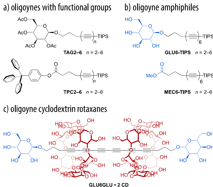
Figure 1. a) Oligoyne derivatives TAG2-6 and TPC2-6 with glycoside and carboxylate functional groups can be deprotected to obtain b) the corresponding amphiphilic oligoyne derivatives GLU6-TIPS and MEC6-TIPS . These may either be used to prepare carbon-rich colloidal aggregates or c) oligoyne cyclodextrin rotaxanes GLU6GLU · 2 CD .
