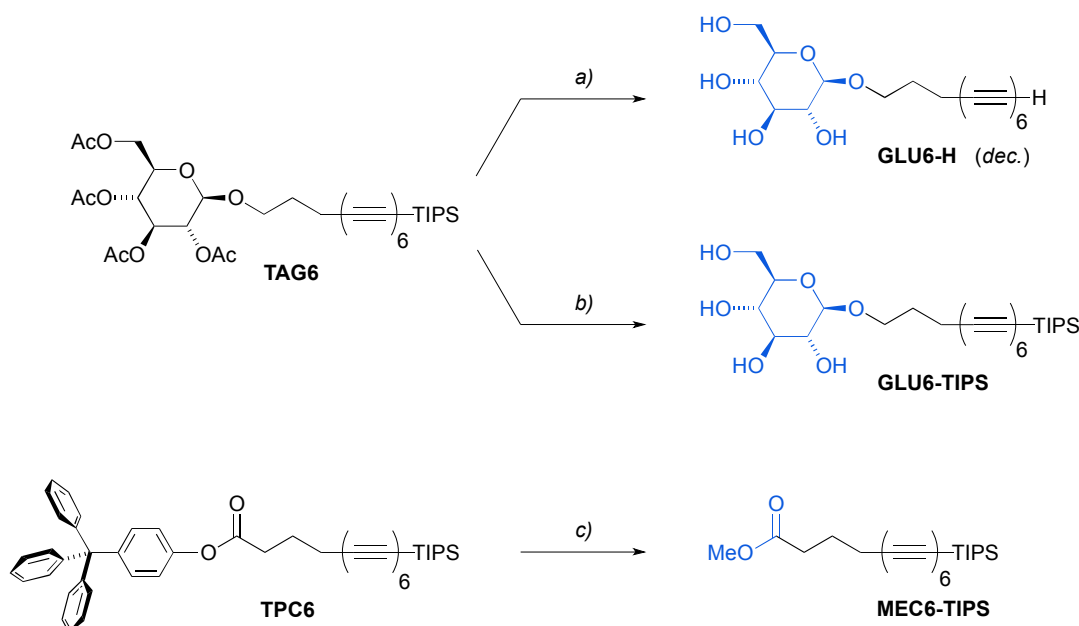
Scheme 3. Synthesis of oligoyne amphiphiles. Reagents and conditions: a) CsF, NaOMe, dioxane/MeOH, r.t., 2 h; b) NaOMe, dioxane/MeOH, r.t., 2 h; then Amberlite (H + ), 30 min; c) NaOMe, DCM/MeOH, r.t., 5 h; then Amberlite (H + ), 1 h. Conversions were quantitative in all cases, but the products were kept in solution and isolated yields not determined.
