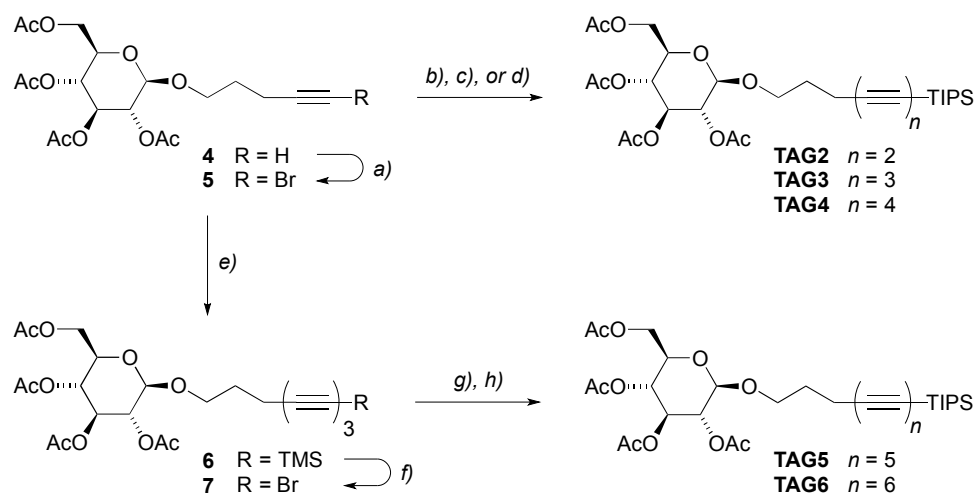
Scheme 1. Synthesis of glycosylated oligoynes TAG2-6 up to the hexaynes. Reagents and conditions: a) \text{AgNO}_3 , NBS, MeCN, 93%; b) \text{TIPS-C}\equiv\text{C-ZnCl } \mathbf{1} , \text{PdCl}_2(\text{dppf}) \cdot \text{DCM} , THF/toluene, 87%; c) \text{TIPS-(C}\equiv\text{C)}_2\text{-ZnCl } \mathbf{2a} , \text{PdCl}_2(\text{dppf}) \cdot \text{DCM} , THF/toluene, 78%; d) \text{TIPS-(C}\equiv\text{C)}_3\text{-ZnCl } \mathbf{3} , \text{PdCl}_2(\text{dppf}) \cdot \text{DCM} , THF/toluene, 51%; e) \text{TMS-(C}\equiv\text{C)}_2\text{-ZnCl } \mathbf{2b} , \text{PdCl}_2(\text{dppf}) \cdot \text{DCM} , THF/toluene, 72%; f) \text{AgF} , NBS, MeCN, 81%; g) \text{TIPS-(C}\equiv\text{C)}_2\text{-ZnCl } \mathbf{2a} , \text{PdCl}_2(\text{dppf}) \cdot \text{DCM} , THF/toluene, 42%; h) \text{TIPS-(C}\equiv\text{C)}_3\text{-ZnCl } \mathbf{3} , \text{PdCl}_2(\text{dppf}) \cdot \text{DCM} , THF/toluene, 55%.
