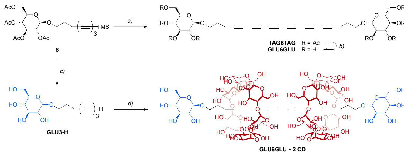
Scheme 4. Synthesis of hexayne rotaxane GLU6GLU · 2 CD and hexayne GLU6GLU . Reactions and conditions: a) CsF, THF/H 2 O; then Cu(OAc) 2 , 2,6-Lutidine, DCM, 73%; b) NaOMe, 1,4-Dioxane/MeOH (5:1), r.t., 3 h (yield not determined); c) NaOMe, Et 2 O/MeOH (4:1), r.t., 2 h; then Amberlite (H + ) (product not isolated); d) \alpha -cyclodextrin (0.1 M in H 2 O), 45 °C, 3 h; then CuBr 2 , TMEDA, r.t., 2 d, 21% over two steps.
