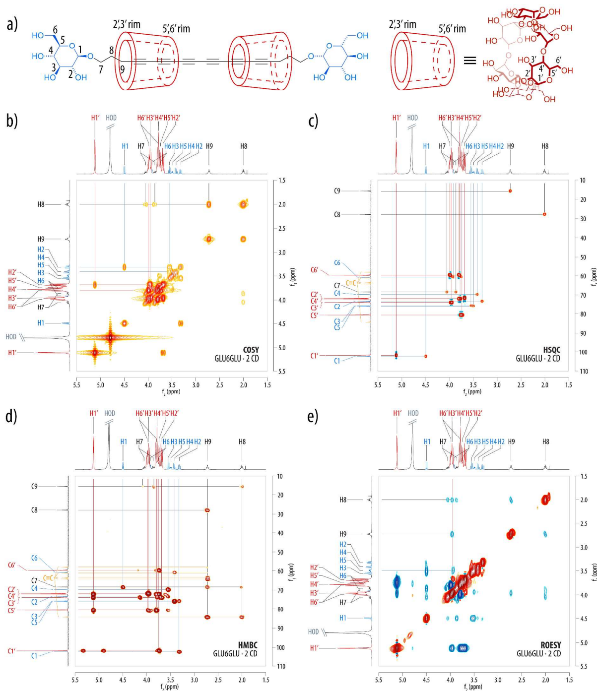
Figure 8. Structure of the [3]rotaxane GLU6GLU · 2 CD and the corresponding 2D NMR spectra (all 400 MHz, 297.2 K, D 2 O). a ) The proposed structure features a tail-to-tail arrangement of the two threaded \alpha -cyclodextrin hosts. The assignment of the signals in the ^1\text{H} and ^{13}\text{C} -NMR spectra was established by means of b ) the ^1\text{H}, ^1\text{H} -COSY NMR spectrum, c ) the ^1\text{H}, ^{13}\text{C} -HSQC NMR spectrum, and d ) the ^1\text{H}, ^{13}\text{C} -HMBC NMR spectrum. e ) The ^1\text{H}, ^1\text{H} -ROESY NMR spectrum of the [3]rotaxane GLU6GLU · 2 CD revealed through-space contacts between H3' of the wider 2,3-rim of the \alpha -cyclodextrin host with the protons H9, H8, and H3 of the hexayne glycosyl host. See Supplementary Figures S1–S4 for enlarged versions and further details.
