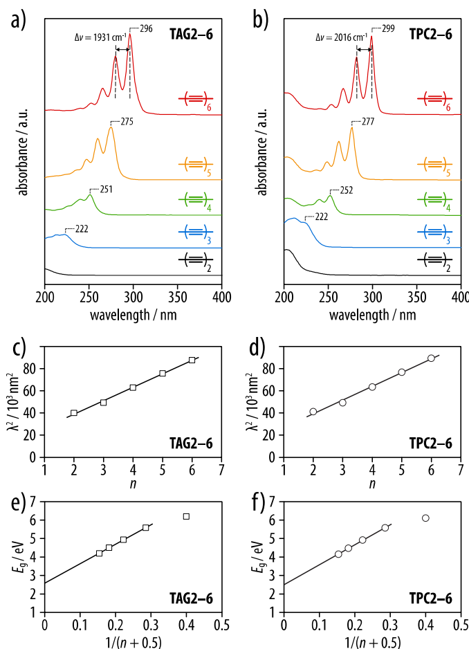
Figure 2. a) UV-Vis spectra of the tetra- O -acetyl \beta -D-glucosyl oligoynes TAG2-6 in acetonitrile (concentrations in the range of c = 3.03 – 4.21 \mu\text{mol/L} ), and b) of the corresponding tritylphenyl carboxylates TPC2-6 in cyclohexane (concentrations in the range of c = 5.86 – 6.55 \mu\text{mol/L} ). c,d) Lewis-Calvin plots of the UV-Vis absorption maxima of the two series with linear regressions with slopes of k = 12.2 \square 10^3 and 12.4 \square 10^3 \text{ nm}^2 ( R^2 = 0.996 and 0.991 ). e,f) Plots of the energy of the optical transition versus 1/(n+0.5) , with the number of triple bonds n . An extrapolation of the linear regression to n = \infty yields values of 480 nm (2.6 eV) and 498 nm (2.5 eV), respectively, for the saturation wavelength of an infinitely long chain of conjugated triple bonds ( R^2 = 0.999 in both cases).
