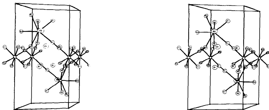
FIG. 2. \text{SmFe(CN)}_6 \cdot 4\text{H}_2\text{O} . A stereodrawing of the unit cell and its contents. The metal ions are shown fully coordinated. The Sm–N≡C–Fe linkages from the edges of distorted cubic cages in which water molecules O(1)'s are trapped.
