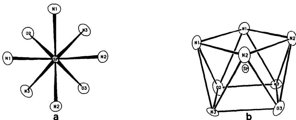
FIG. 1. \text{SmFe(CN)}_6 \cdot 4\text{H}_2\text{O} . The atoms Sm, O(2), and O(3) occupy a crystallographic mirror plane. (a) A top view of the square antiprismatic geometry ( D_{4d} ). (b) A regular presentation of a square antiprism.
