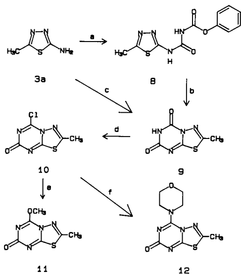
Scheme 2. a: \text{PhOCON}=\text{C}=\text{O}/\text{CH}_3\text{CN}/\text{heat} 2 hours. b: xylenes/heat 6 hours. c: \text{PhO-CO-N}=\text{C}=\text{O}/\text{xylenes}/\text{heat} 16 hours. d: \text{PCl}_5/\text{POCl}_3 . e: \text{CH}_3\text{OH}/\text{heat} 30 minutes. f: morpholine/room temperature.
