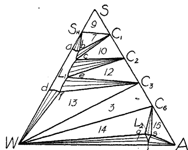
Fig. 13.—Isotherm at binary eutectic \gamma , -11.7^{\circ} (schematic).
