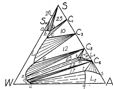
Fig. 22.—Isotherm above quintuple point H, +42^\circ (schematic).
