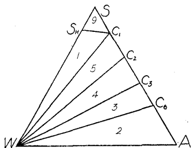
Fig. 5.—Isotherm below -58.8^{\circ} (schematic).
