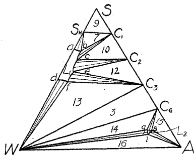
Fig. 12.—Isotherm above quintuple point D, -12^{\circ} (schematic).
