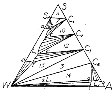
Fig. 15.—Quintuple point E, -0.67^{\circ} (schematic).
