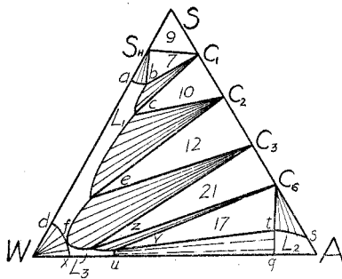
Fig. 20.—Consolute temperature \beta , -0.04^\circ (schematic).
