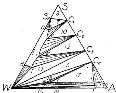
Fig. 16.—Isotherm above quintuple point E (schematic).
