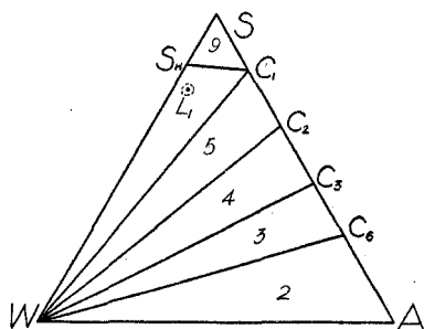
Fig. 6.—Quintuple point A, -58.8^{\circ} (schematic).
