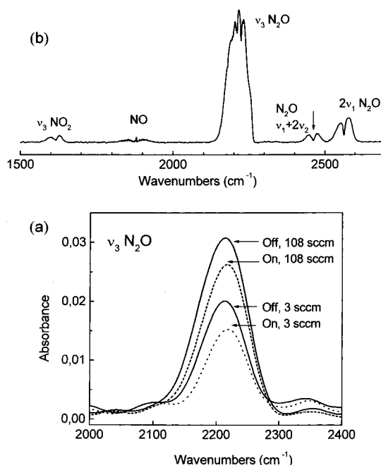
Figure 2. (a) Absorbance spectra of the \nu_3 band of N 2 O with a spectral resolution of 40 cm -1 , at two different moments, with discharge “on” and “off”, and at the two different values of N 2 O gas flow rates (3 and 108 sccm). Integration of the band was performed between 2100 and 2300 cm -1 for obtaining the concentration. (b) FTIR rapid-scan spectrum of a DC, 40 mA, 3 sccm, N 2 O discharge between 1500 and 2700 cm -1 with a spectral resolution of 2 cm -1 . Some weak bands of NO and NO 2 , as well as the 2\nu_1 and \nu_1 + 2\nu_2 bands of N 2 O can be observed.
