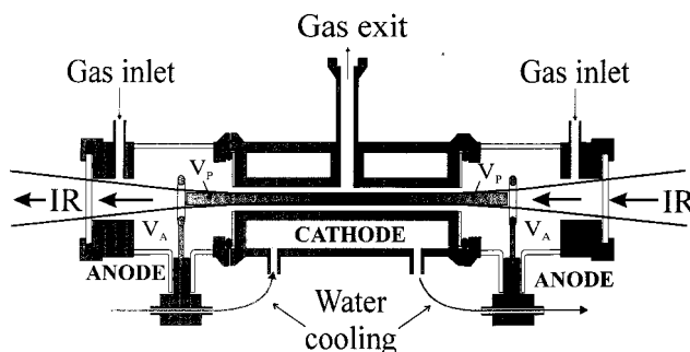
Figure 1. Scheme of the hollow cathode discharge cell, showing the focusing and the optical path of the IR beam of the FTIR spectrometer across the cell, as well as the location of the plasma region, V_P , and of the rest of the volume without electrical charge, V_A , assumed in the present theoretical model. Mass spectrometry is performed in this cell by replacing one of the IR windows by a flange supporting a central diaphragm with a diameter of 100 \mu\text{m} . Another flange holding the double Langmuir probe can be used in order to measure the charge density and mean electron energy.
