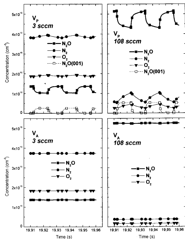
Figure 4. Theoretical predictions of the time dependent concentrations of the major products of the discharge \text{N}_2\text{O} , \text{N}_2 and \text{O}_2 in the two volumes V_p and V_A considered in the present model, with the hollow cathode discharge cell operating at 45 Hz and 2 mbar, for the two gas flow rates, 3 and 108 sccm. The behavior of the (001) vibrational excited level of \text{N}_2\text{O} in the plasma volume is shown too.
