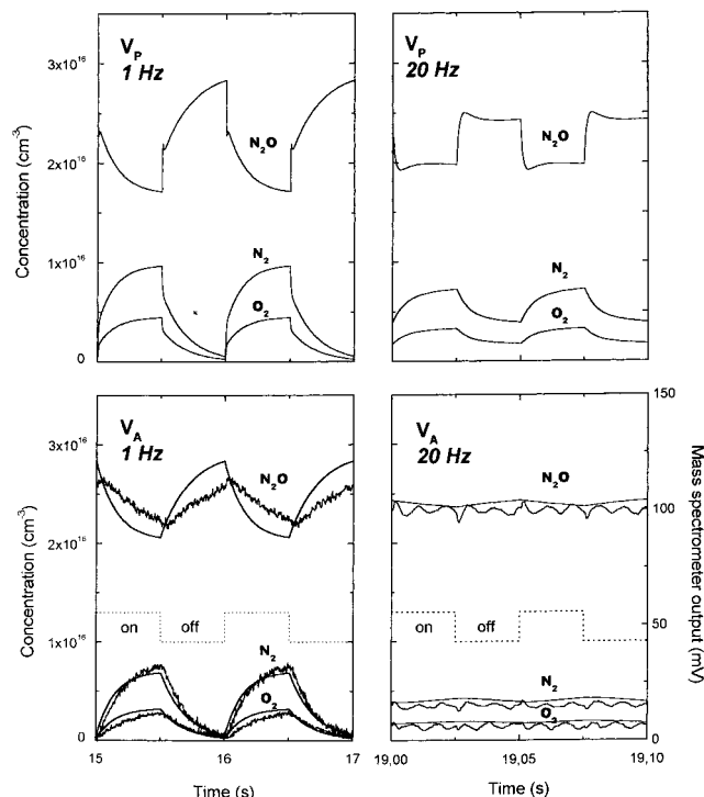
Figure 5. Mass spectrometer outputs in mV of \text{N}_2\text{O} (44 amu), \text{N}_2 (28 amu) and \text{O}_2 (32 amu) sampled at one edge of the discharge cell, drawn at modulation frequencies of 1 Hz (left-bottom panel) and 20 Hz (right-bottom panel) for a 1 mbar, 36 sccm, 100 mA discharge and compared with the absolute concentration values predicted in V_A by the present theoretical model. In the upper panels, the theoretical predictions of the behavior of \text{N}_2\text{O} , \text{N}_2 and \text{O}_2 inside the plasma volume, V_p , are shown too.
