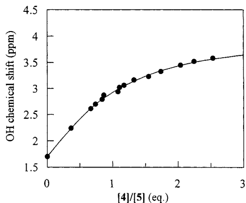
Fig. 2 ^1\text{H} NMR (500 MHz) titration data and the simulated curve fit for 4 binding 5 in \text{CDCl}_3 , monitoring the hydroxy proton of 5 .
