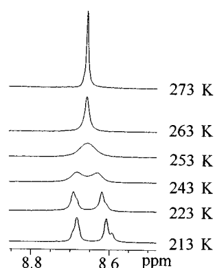
Fig. 3 VT ^1\text{H} NMR (400 MHz) spectra of the aromatic protons of 4 in \text{CDCl}_3 .
