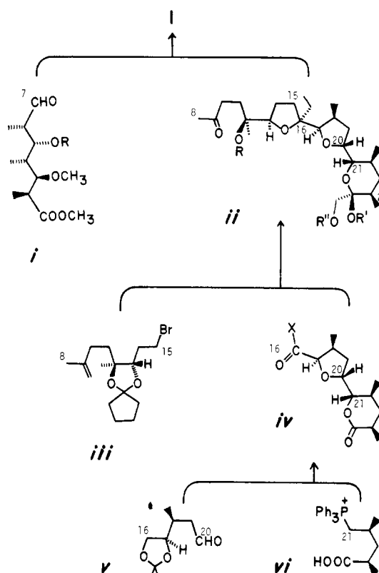
Scheme I
