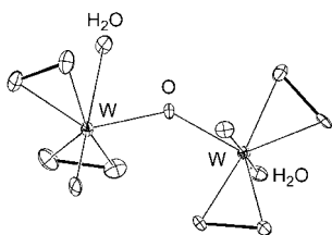
Figure 1. Molecular structure of the anion part of K_2\{[W(=O)(O_2)_2(H_2O)_2(\mu-O)]_2(H_2O)_2\} \cdot 2H_2O ( I ).
