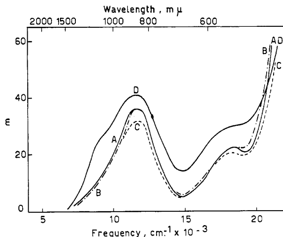
Figure 1.—Absorption and reflectance spectra of [SALen-NHCH_3]_2Ni complex at room temperature: A, in benzene; B, in pyridine; C, in chloroform; D, reflectance spectrum.
