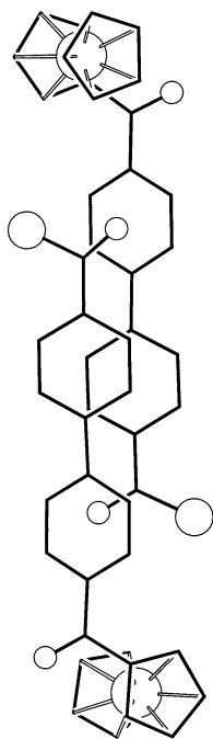
Fig. 3. View of one pair of \pi -stacked molecules, formed by molecules of types 1 and 3, showing the ring offset approximately equal to the radius of an aryl ring. For the sake of clarity, only the major conformation of the chlorocarbonyl groups is shown, and H atoms are omitted.
