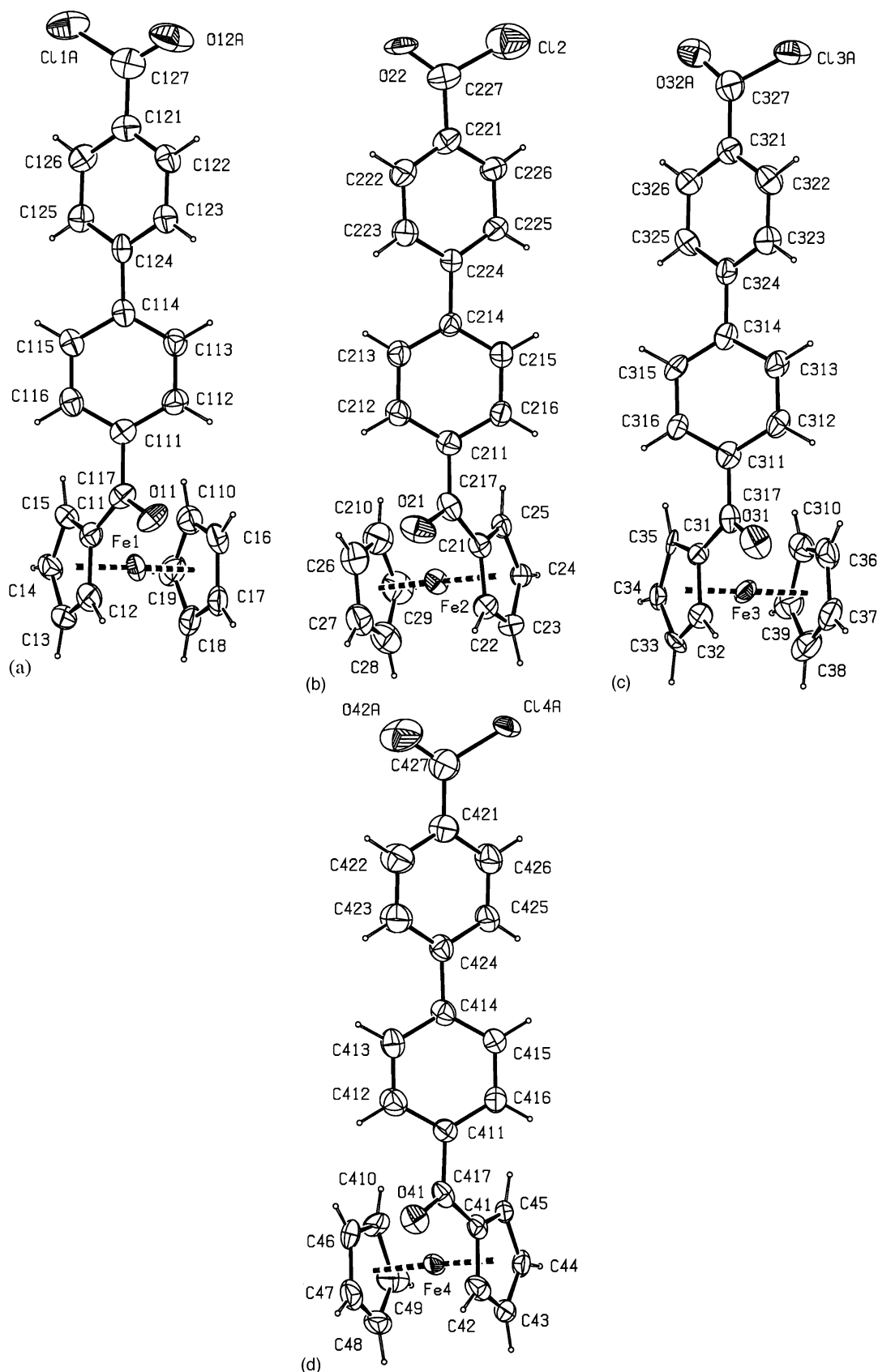
Fig. 1. Views of the four independent molecules in the crystal structure of 1a , showing the atom-labelling scheme and the rotational disorder of the chlorocarbonyl groups in molecules 1, 3 and 4. Displacement ellipsoids are drawn at the 30% probability level.
