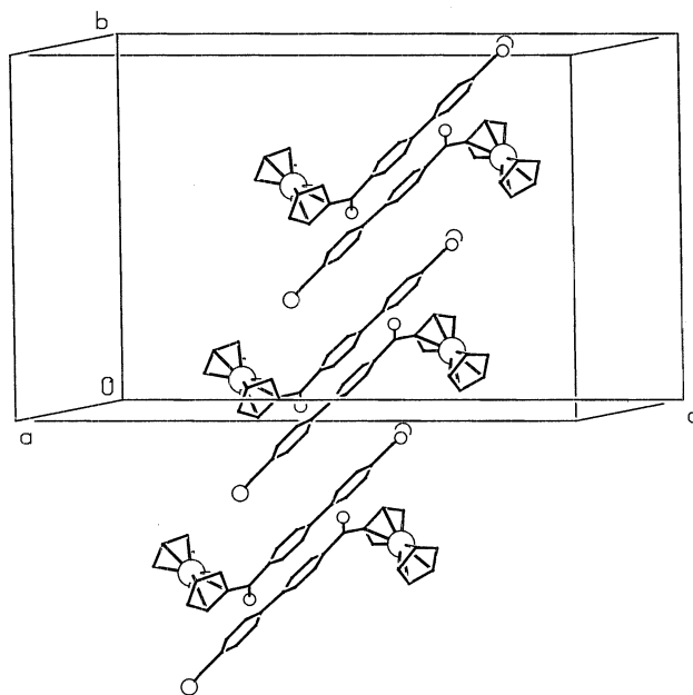
Fig. 4. View of one of the [1\bar{1}0] chains built from molecules of types 1 and 3: atoms are depicted as in Fig. 3.
