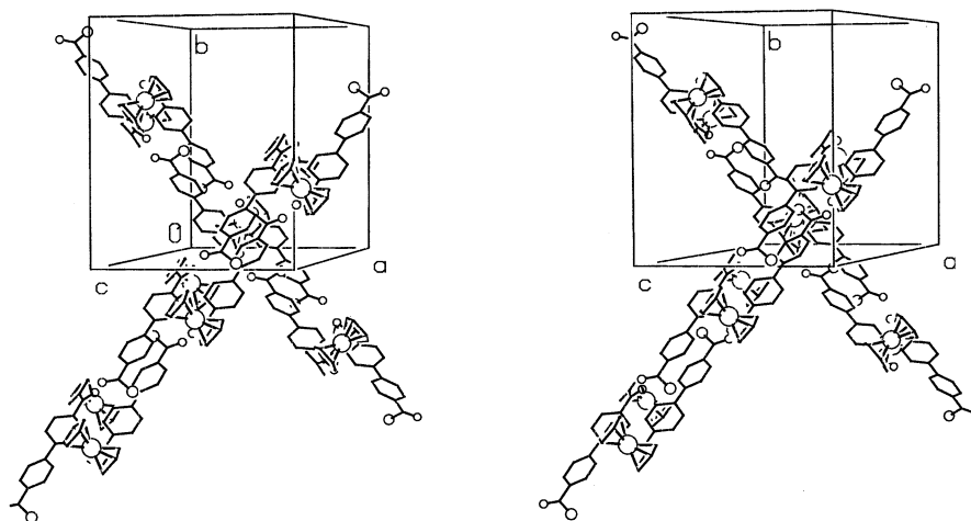
Fig. 5. Stereoview of the stacked [1\bar{1}0] and [110] chains.
