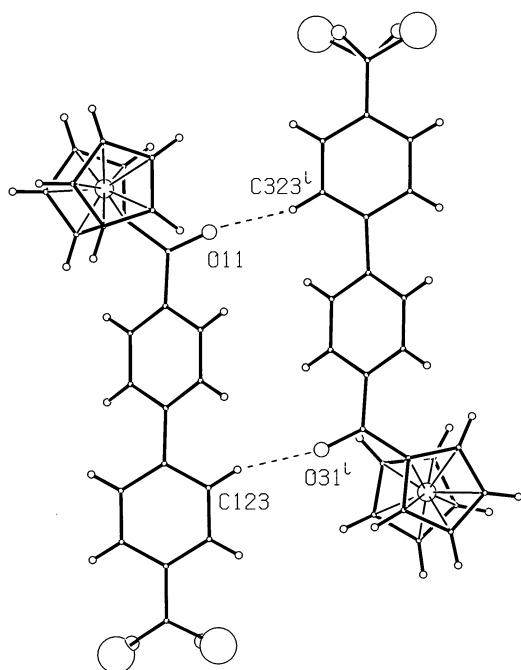
Fig. 2. The cyclic dimer formed by molecules of types 1 and 3, showing the R_2^2(18) ring formed by the two C–H...O hydrogen bonds.
