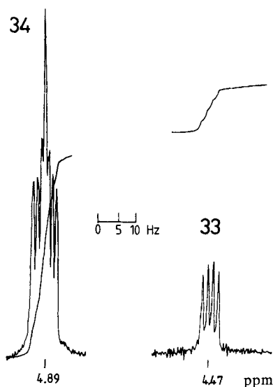
Fig. 5. Partial ^1\text{H} -NMR. (360 MHz, \text{CDCl}_3 ) spectrum of the reaction mixture 18 + TCE \rightarrow 33/34 (15:85). The signals of H-C(3) are shown (compare with those of 29 and 30 , Fig. 4).
