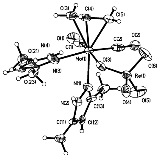
Figure 1. Thermal ellipsoid (30%) plot of cis,cis -[Mo(OReO 3 )(η 3 -allyl)(CO) 2 (Hdmpz) 2 ] ( 3 ).
