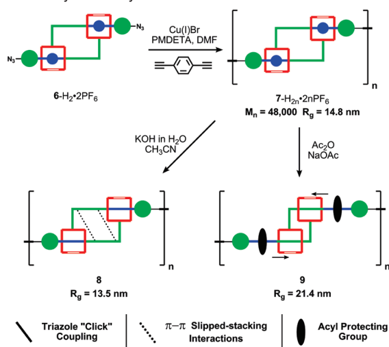
Scheme 2. Graphical Representation Depicting Synthesis of Linear “Click” Polymer 7 -H 2n •2nPF 6 , Decoordinated Polymer 8 a , and Extended Acylated Polymer 9 a
