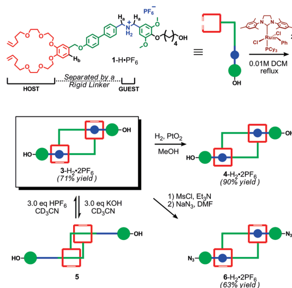
Scheme 1. Graphical Representation of the Synthesis of [c2]Daisy-Chain Dimer 3 -H 2 •2PF 6 , Hydrogenated Derivative 4 -H 2 •2PF 6 , Decoordinated Dimer 5 , and Diazide Analogue 6 -H 2 •2PF 6
