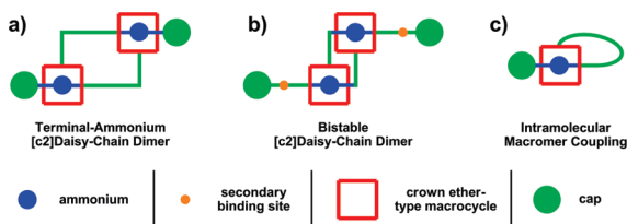
Figure 1. Graphical representation of a [c2]daisy-chain dimer containing adjacent cap and ammonium moieties (a), a bistable [c2]daisy-chain dimer (b), and an intramolecularly coupled macromer (c).
