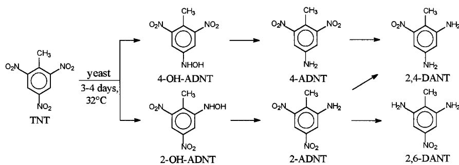
Scheme 1. Reduction pathways from TNT to DANTs
