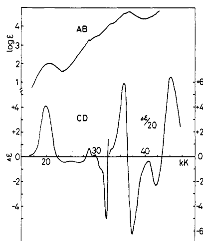
Figure 1. AB and CD spectra for (+)-D-[Co(phen) 2 (Gly)] 2+ .
