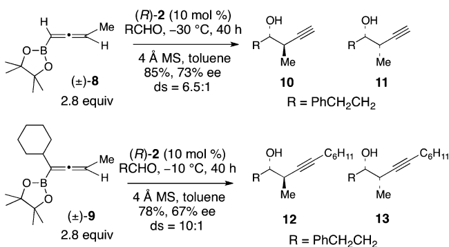
Scheme 4. Kinetic Resolution/Allenylboration Reactions with Racemic Allenylboronates 8 and 9
