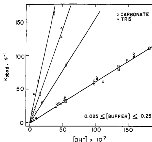
Figure 2. Kinetic data for the hydrolysis of the 2-cyanobenzamide complex at 25.5, 33.0, 38.0, and 43.2 ^\circ\text{C} .
