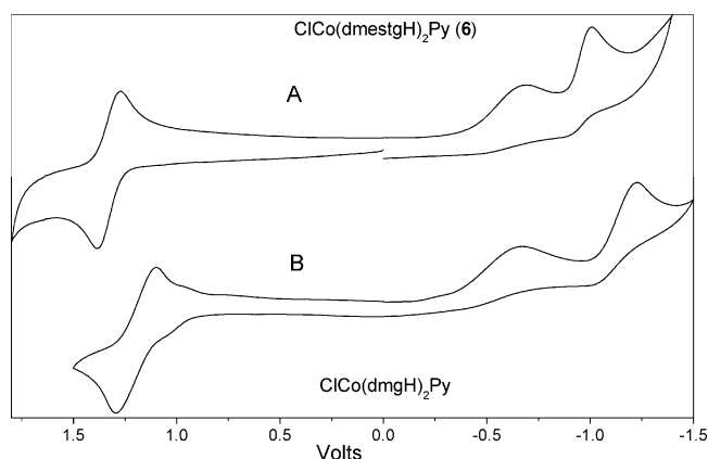
Figure 1. Cyclic voltammograms of 6 (A) and ClCo(dmH) 2 Py (B) in CH 2 Cl 2 with 0.1 M (NBu 4 )PF 6 as supporting electrolyte at 0.2 V s −1 at 25 °C.
