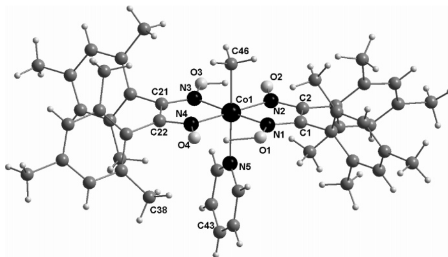
Figure 3. Structure of \text{MeCo}(\text{dmestgH})_2\text{Py} ( 1 ).
