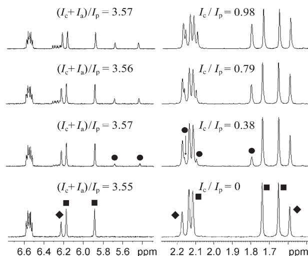
Figure 2. 1 H NMR (300 MHz) spectral changes of 1 in C 6 D 6 solution at 298 K on irradiation, showing the time course of closed-form formation (from bottom to top). The signals corresponding to the antiparallel (■) and parallel (◆) conformations of the open form and the closed form (●) are labeled. ( I_a , I_p , and I_c are the integrals of the methyl protons corresponding to signals of antiparallel and parallel conformations of the open and closed forms, respectively).
