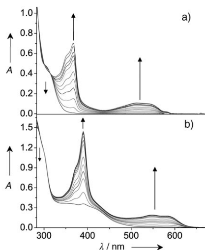
Figure 1. UV/Vis absorption spectral changes of a) L1 ( 5.52 \times 10^{-5} M) and b) 1 ( 7.16 \times 10^{-5} M) in benzene solution on excitation at 313 and 440 nm, respectively.
