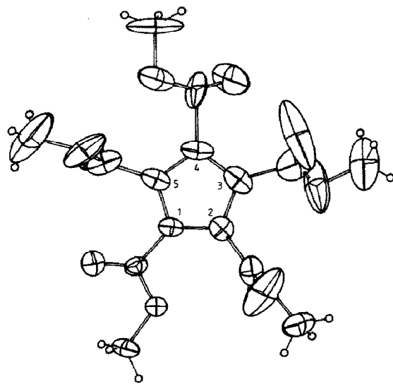
Fig. 3. (a) Unit cell contents of 12 , projected down c . (b) A single cation of 12 , projected normal to the iridium coordination plane. (c) The cpp anion of 12 , projected normal to the C_5 plane.
