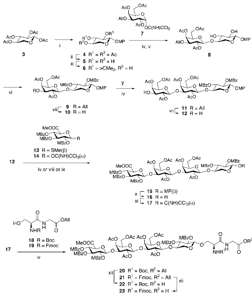
Scheme 1: Reagents and conditions: i) 4-methoxyphenol, TMSOTf, MS4A, \text{CH}_2\text{Cl}_2 , -20^\circ\text{C} , 1 h; ii) \text{Et}_3\text{N} , MeOH, \text{H}_2\text{O} , rt, overnight; iii) 2-methoxypropene, camphorsulfonic acid, DMF, 60^\circ\text{C} , 5 h; iv) TMSOTf, MSAW300, \text{CH}_2\text{Cl}_2 , -20^\circ\text{C} , 1 h; v) camphorsulfonic acid, MeOH, \text{CH}_2\text{Cl}_2 , rt, 2 h; vi) 4-methylbenzoyl chloride, pyridine, rt, 1.5 h; vii) (1,5-cyclooctadiene)bis(methyldiphenylphosphine)iridium(I) hexafluorophosphate, THF, \text{H}_2 , then \text{I}_2 , \text{H}_2\text{O} , \text{NaHCO}_3 , rt, 2.5 h; viii) \text{BF}_3 \cdot \text{OEt}_2 , MSAW300, \text{CH}_2\text{Cl}_2 , -20^\circ\text{C} \sim \text{rt} , overnight; ix) \text{CuBr}_2 , AgOTf, n - \text{Bu}_4\text{NBr} , MS4A, \text{CH}_2\text{Cl}_2 , 0^\circ\text{C} \sim \text{rt} , overnight; x) CAN, \text{CH}_3\text{CN} , \text{H}_2\text{O} , 0^\circ\text{C} , 4 h; xi) \text{CCl}_3\text{CN} , DBU, \text{CH}_2\text{Cl}_2 , 0^\circ\text{C} , 2 h; xii) (\text{Ph}_3\text{P})_4\text{Pd}(\text{O}) , N -methylaniline, THF, rt, 4 h.
