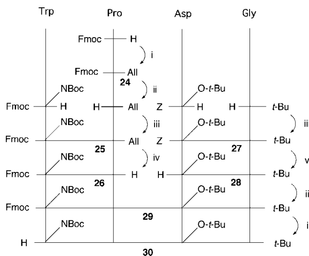
Scheme 2: Reagents and conditions: i) \text{Cs}_2\text{CO}_3 , EtOH, rt, 1 h, then \text{AlIBr} , DMF, rt, overnight; ii) Morpholine, \text{CH}_2\text{Cl}_2 , rt, overnight; iii) HOBt, HBTU, \text{CH}_2\text{Cl}_2 , -20^\circ\text{C} \sim \text{rt} , overnight; iv) (\text{Ph}_3\text{P})_4\text{Pd}(\text{O}) , N -methylaniline, THF, rt, 15 h; v) \text{Pd-C} , \text{H}_2 , MeOH, AcOH, rt, 3 h.
