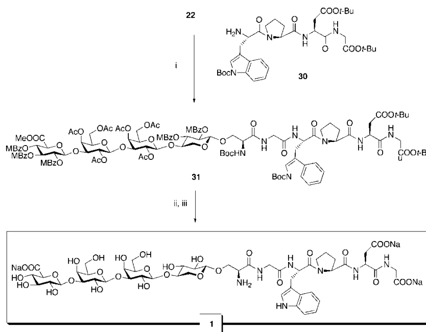
Scheme 3: Reagents and conditions: i) HOBt, HBTU, i -Pr 2 EtN, DMF, −20°C ~rt, overnight; ii) TFA, thioanisole, phenol, H 2 O, 1,2-ethanedithiol, trisopropylsilane, CH 2 Cl 2 , rt, 2 h; iii) NaOMe, MeOH, H 2 O, rt, 3 h.
