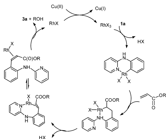
Scheme 3. Plausible Mechanism for the Formation of Quinolones
