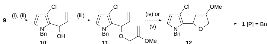
Scheme 4 Reagents: (i) NaH, BnBr, THF (74 %); (ii) vinyl-MgBr, THF; (iii) NaH, 2-methoxyallyl bromide, 13 THF (80–92 % two steps); (iv) \text{Cl}_2(\text{Cy}_3\text{P})_2\text{Ru}=\text{CHPh} (0.2 equiv.), \text{CH}_2\text{Cl}_2 ; (v) 'Mo-F6' (0.2–1.0 equiv.), hexane.
