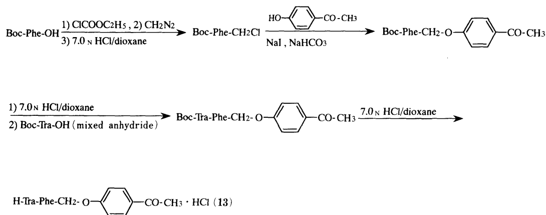
Fig. 2. Synthetic Route to H-Tra-Phe-4-Acetylphenoxymethyl Ketone
